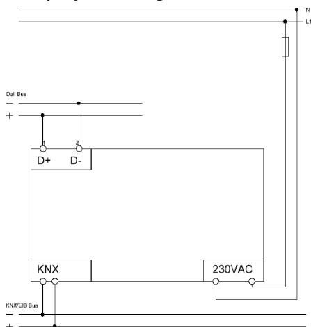
Exemplary circuit diagram SCN-DALI16.03
