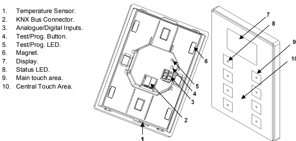
Figure 3 Element diagram.
