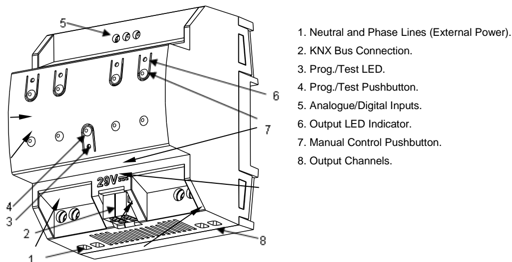
Figure 3 DIMinBOX DX2 - Element Diagram.
