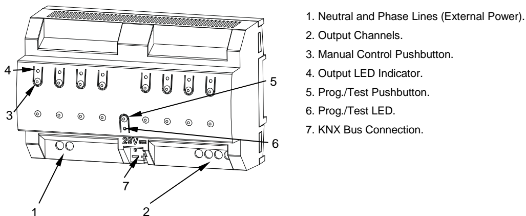
Figure 4 DIMinBOX DX4 - Element Diagram.
