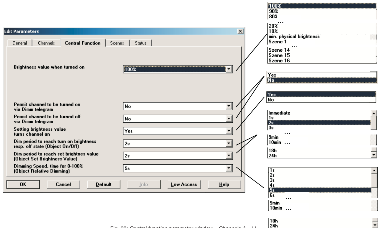
Fig. 23: Central function parameter window – Channels A....H
