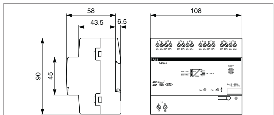
Fig. 5: DALI-Gateway DG/S 8.1, Dimension drawing
