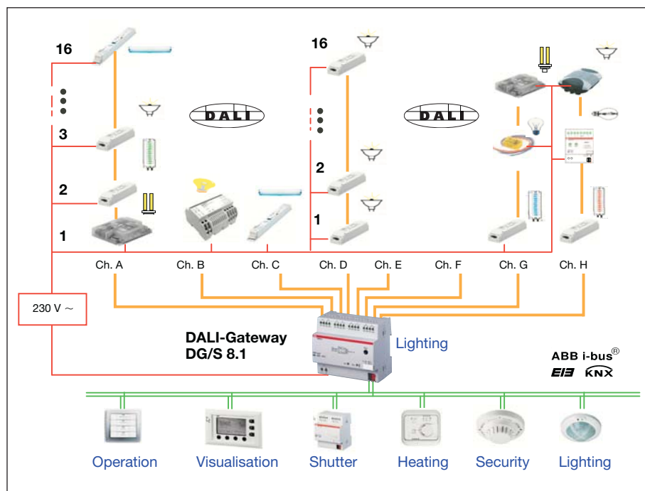
Fig. 6: DALI-Gateway DG/S 8.1, Connection diagram
