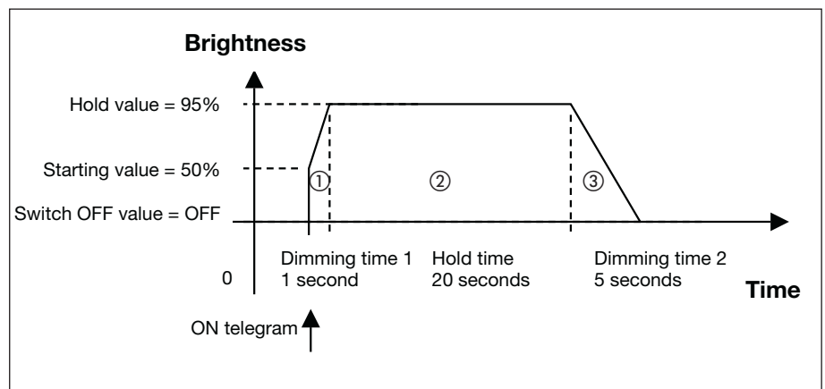
Fig. 30: Timed progression of the staircase lighting function
