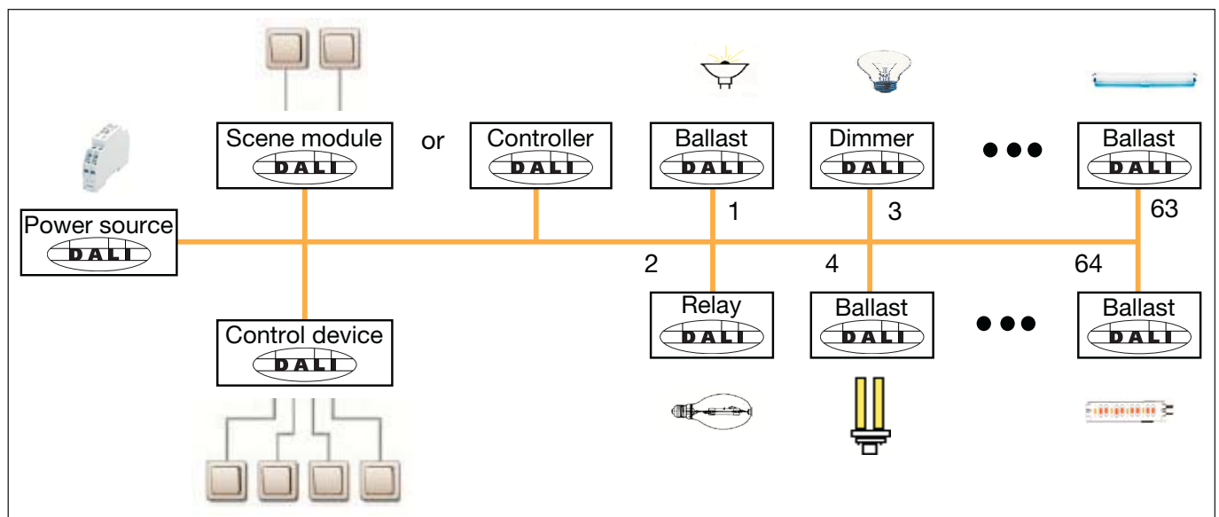
Fig. 2: DALI block diagram
