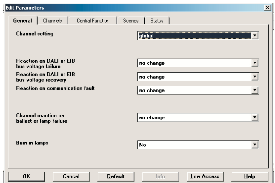
Fig. 16: First parameter window when “Edit Parameters” dialog is retrieved (default setting)
