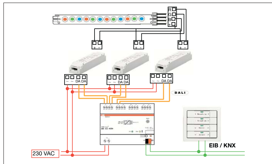
Fig. 28: Example of colour LED system
