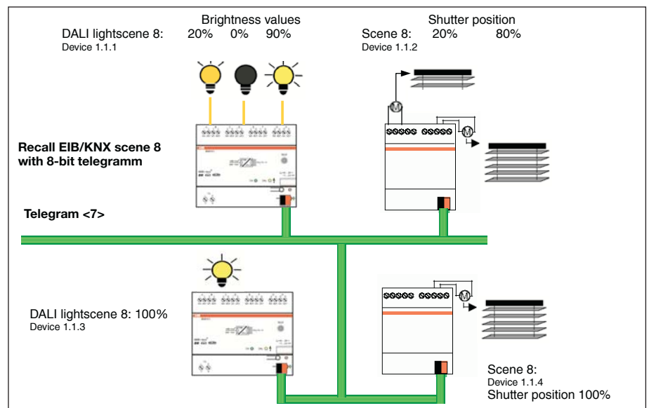
Fig. 27: 8-bit-scene example: Recall scene no. 8
