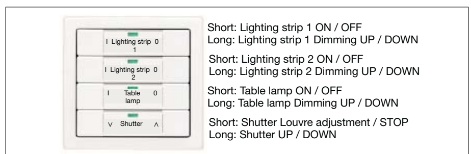
Fig. 33: Push button assignment for “Individual solution”
