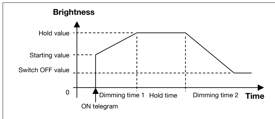
Fig. 7: Dynamic mode - Timed progression of the dimming range
