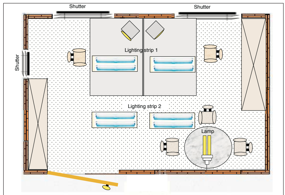
Fig. 32: Office example
