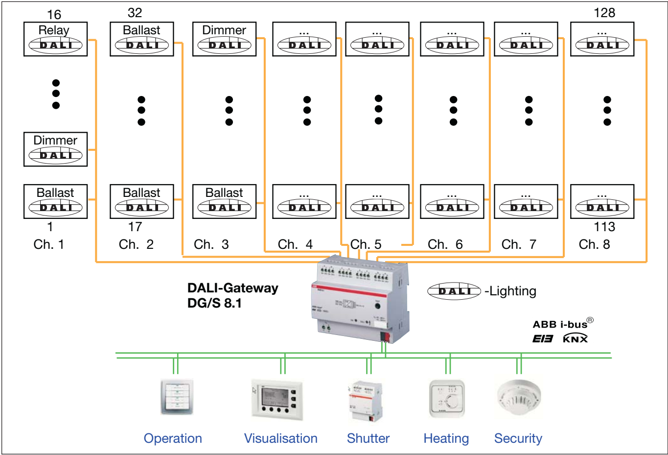
Fig. 3: DALI-Gateway DG/S 8.1, Block diagram
