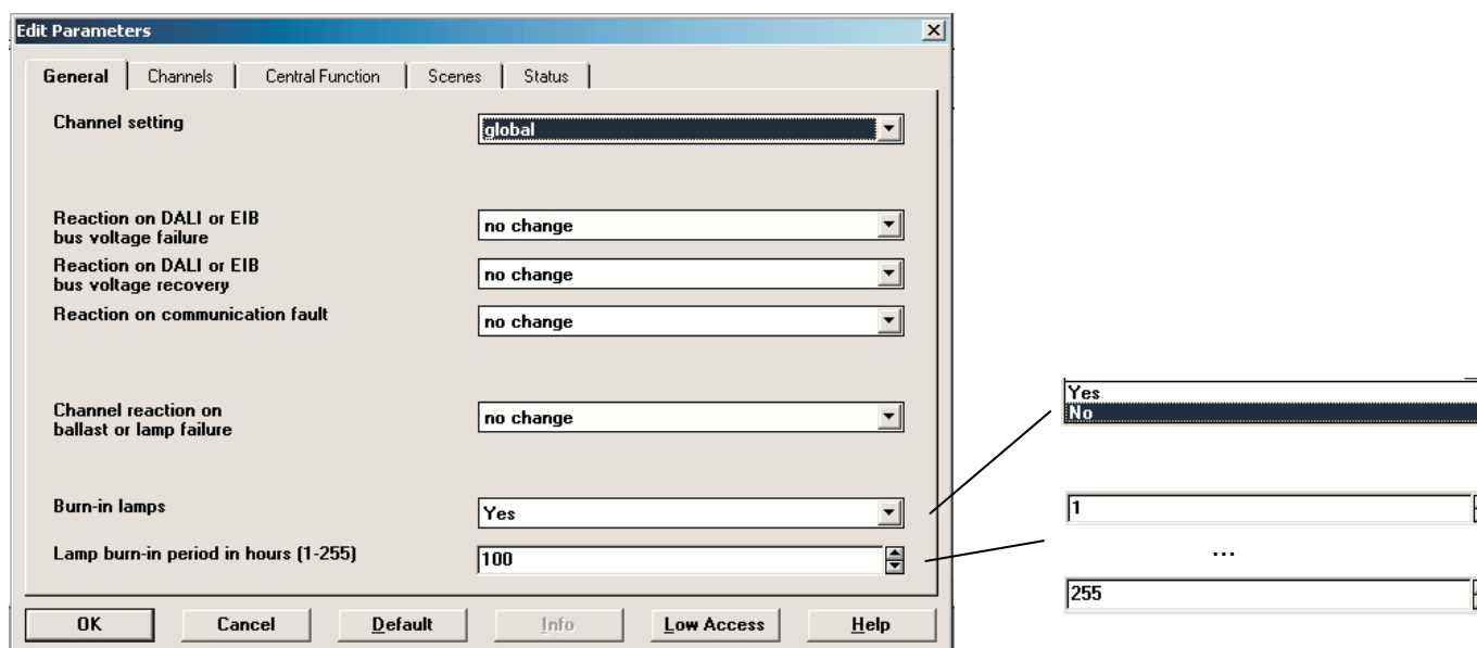
Fig. 19: General parameter window - Burn-in time of lamps
