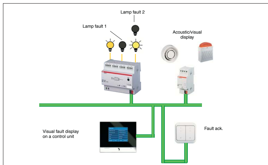
Fig. 31: System representation of a fault signal
