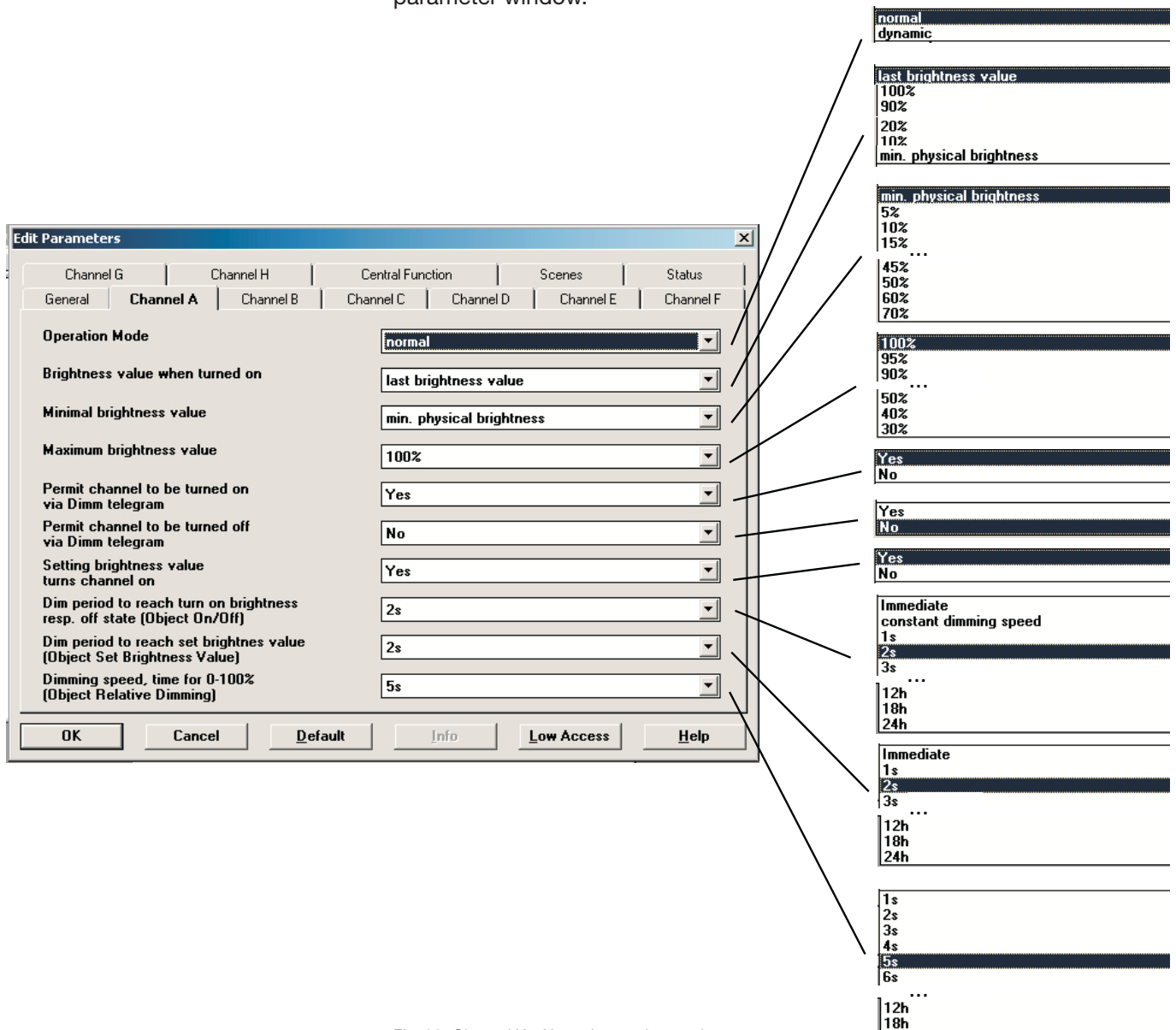
Fig. 20: Channel X – Normal operating mode
