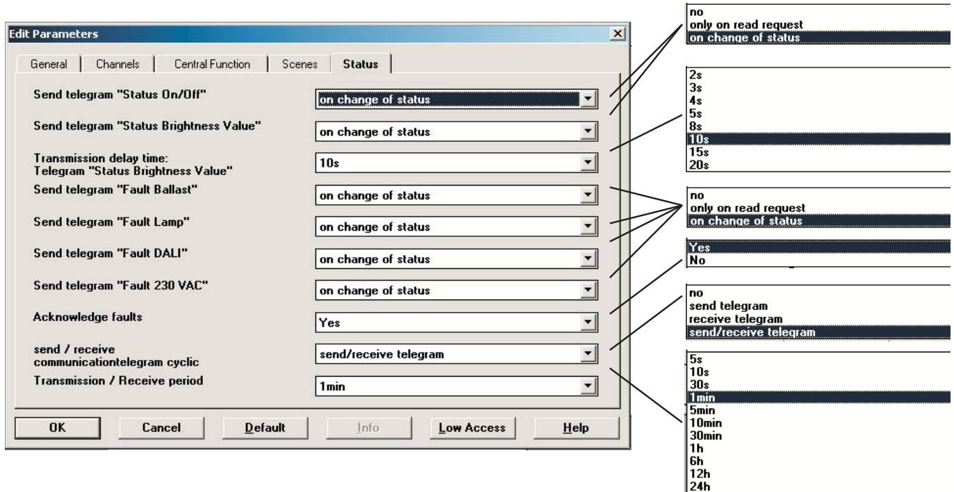
Fig. 26: Status parameter window – Status settings and fault signals
