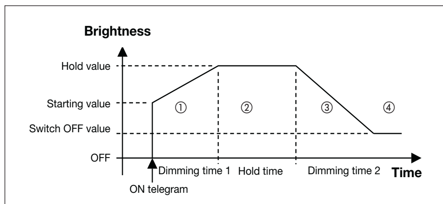
Fig. 22: Graphical representation of dynamic mode
