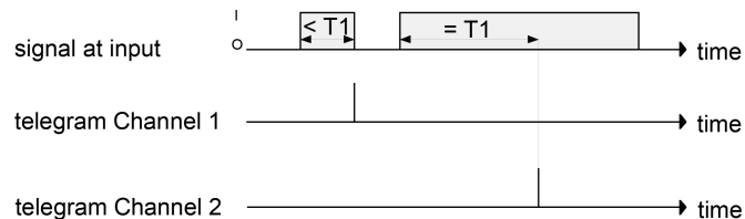
Image 21: Example of operation concept "Channel 1 or Channel 2"
