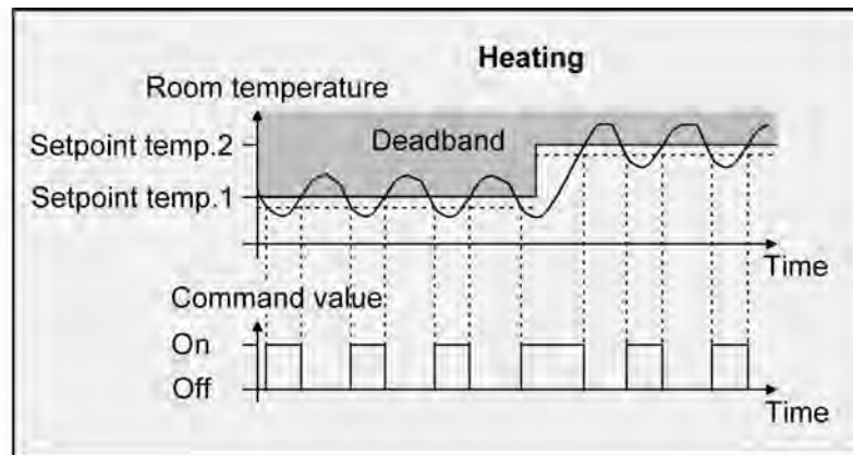
picture 32: 2-point control for mixed "Heating and cooling" mode with active heating operation.
