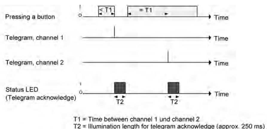
picture 25: Example of operation concept "Channel 1 or Channel 2"
