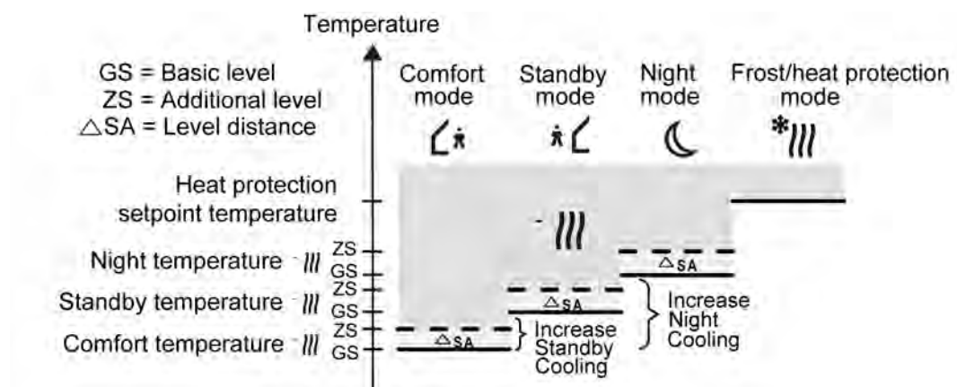
picture 43: Setpoint temperatures in the operating mode "Basic and additional cooling" (recommended specification)
