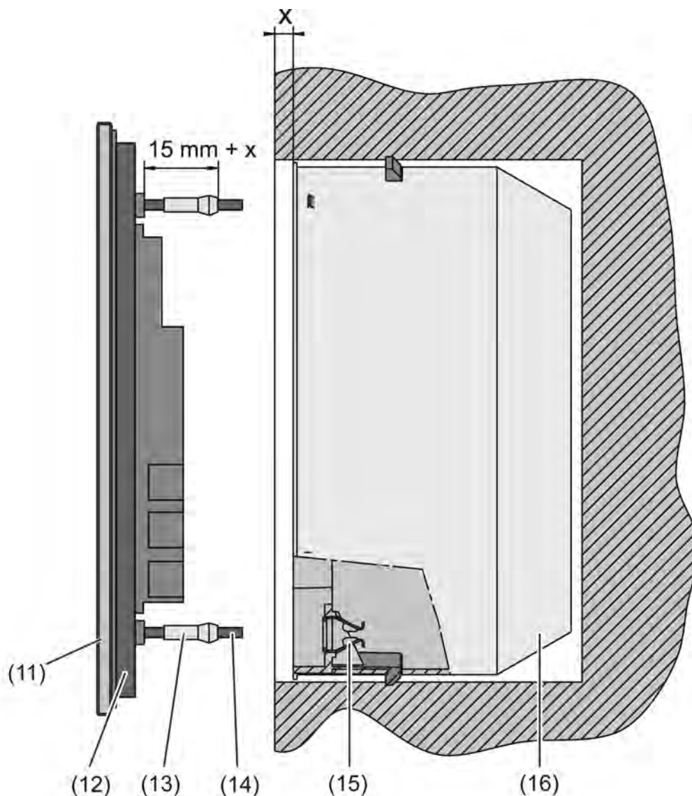
picture 4: Fastening on concealed appliance box
