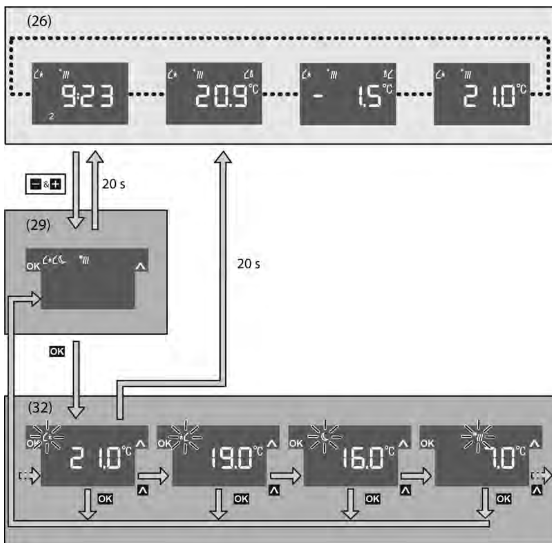
picture 12: Submenu for operating mode selection
