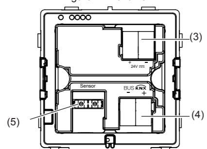
Figure 2: Rear view
