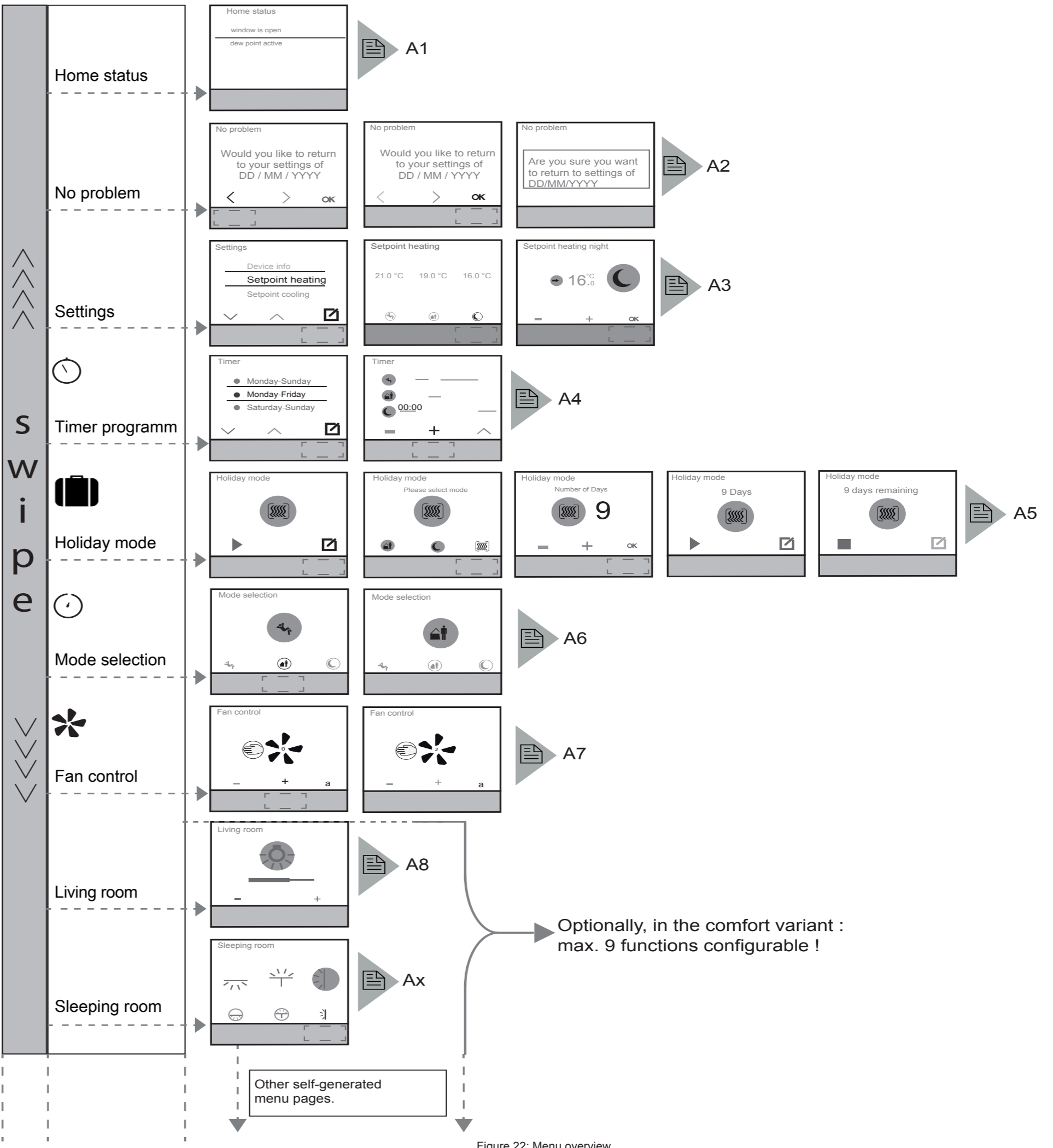
Figure 22: Menu overview
