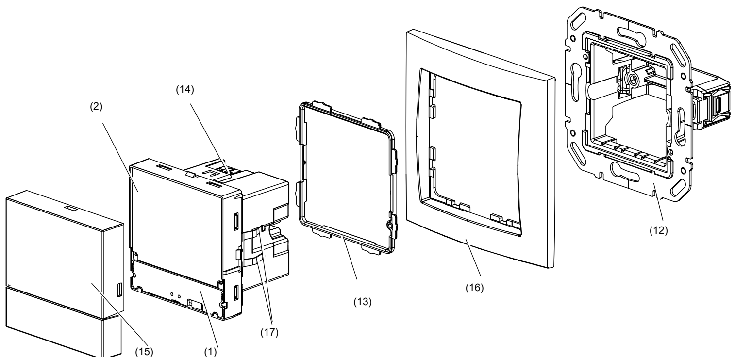
Figure 21: Assembly of the device
