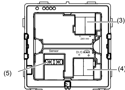
Figure 2: Rear view
