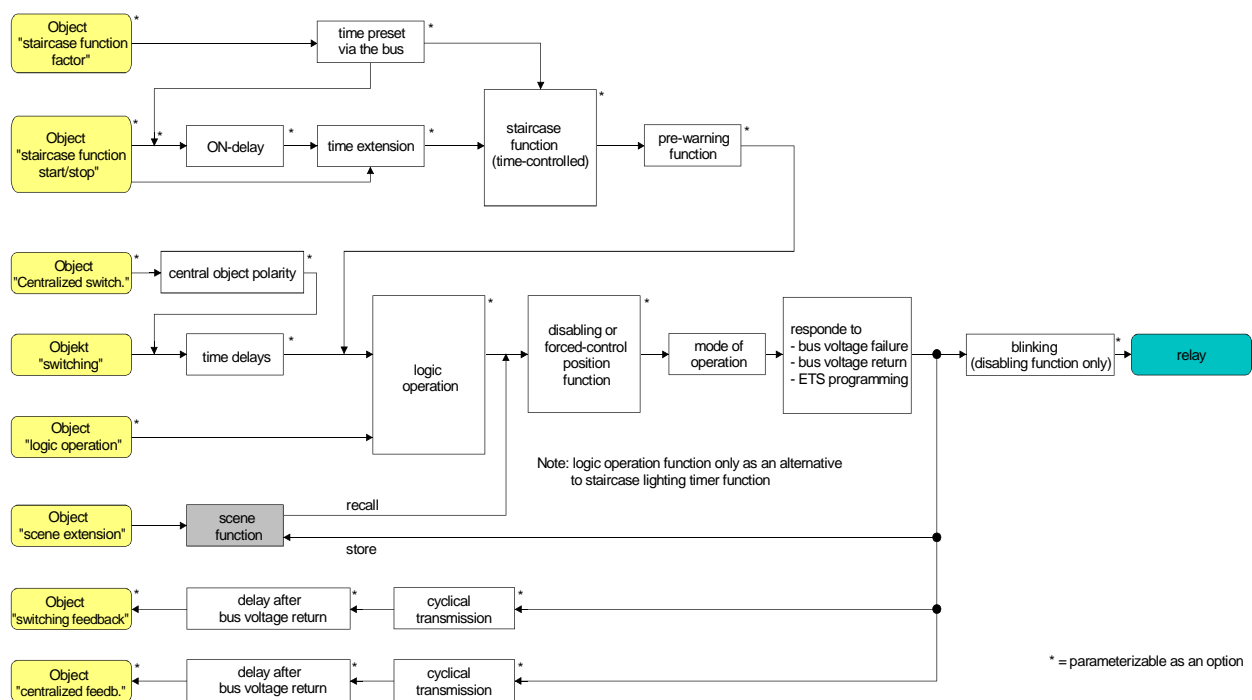
Fig. 15: Functional diagram of the scene function
