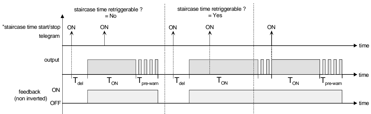
Fig. 11: Switch-on behaviour of the staircase function
