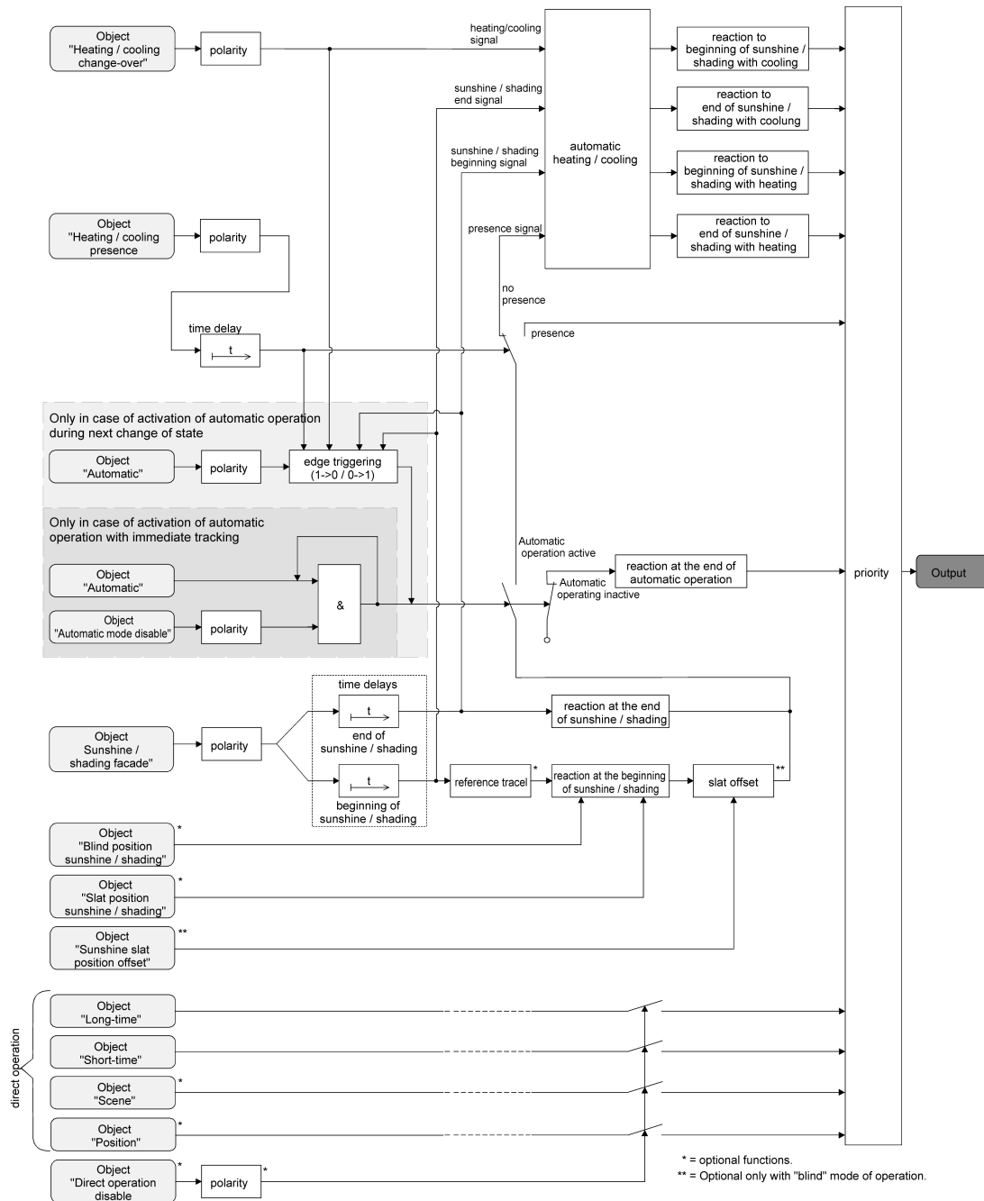
Figure 26: Schematic function diagram of automatic heating/cooling
