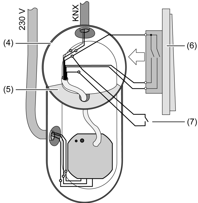
Figure 3: Installing the device in an electronics box (example)
