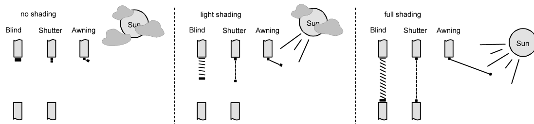
Figure 19: Sun protection principles (example)
