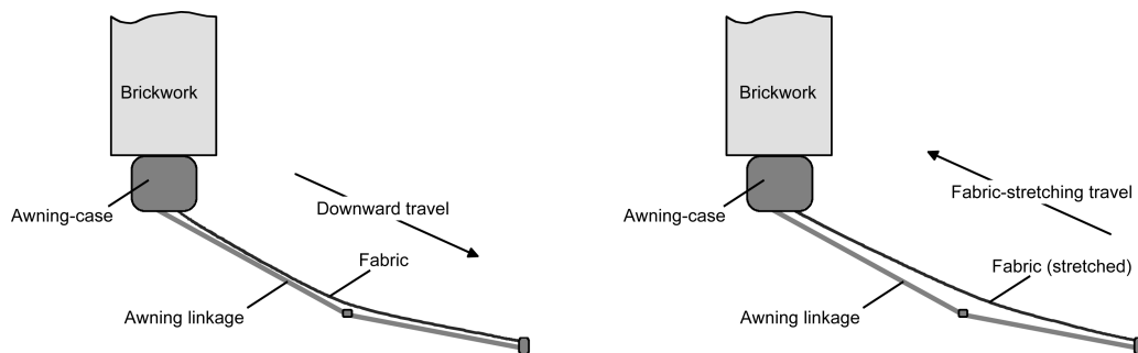
Figure 27: Fabric stretching in an awning
