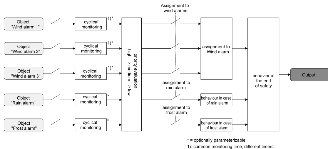
Figure 18: Function diagram of the safety function
