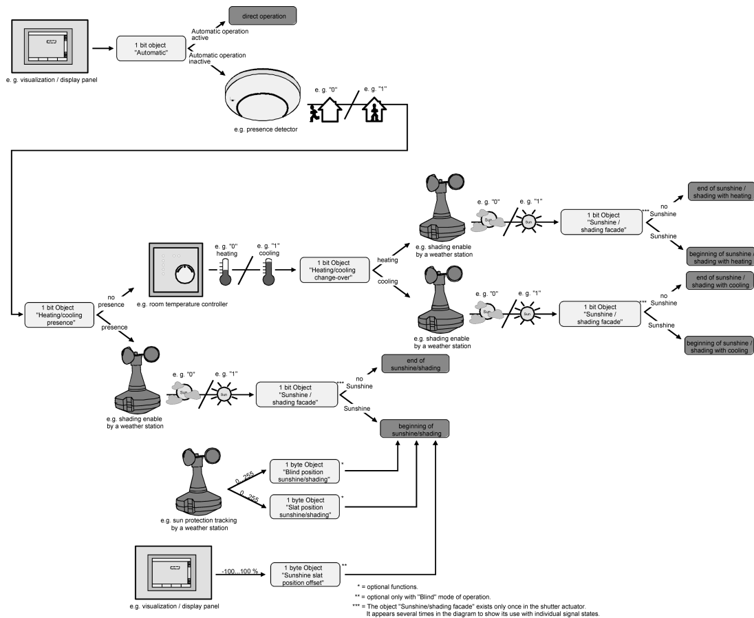
Figure 25: Schematic diagram of automatic heating/cooling (for reasons of simplicity shown without disabling functions of the automatic or direct operation)
