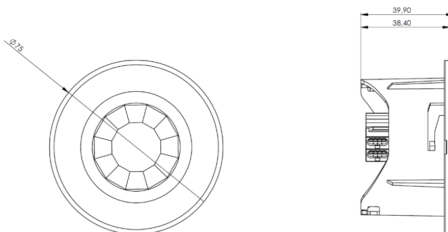
Figure 2: Flush mounted PD100
