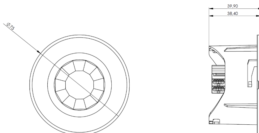
Figure 2: Flush mounted PD100
