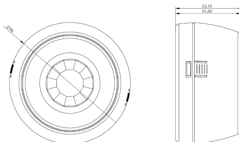
Figure 1: Surface mounted PD100
