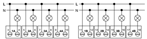
f Connection of the loads (device EK-FE1-TP used as 8-fold binary output)
