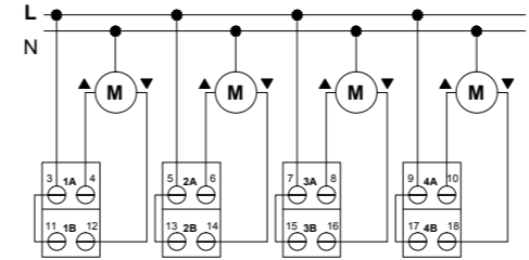
g Connection of the loads (device EK-FE1-TP used as 4-fold blind actuator)
