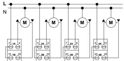
i Connection of the loads (device EK-FF1-TP used as 8-fold blind actuator)
