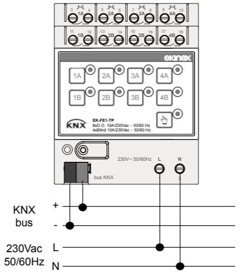
e Connection of the KNX bus network and 230 Vac power supply
