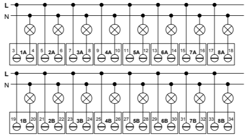
h Connection of the loads (device EK-FF1-TP used as 16-fold binary output)
