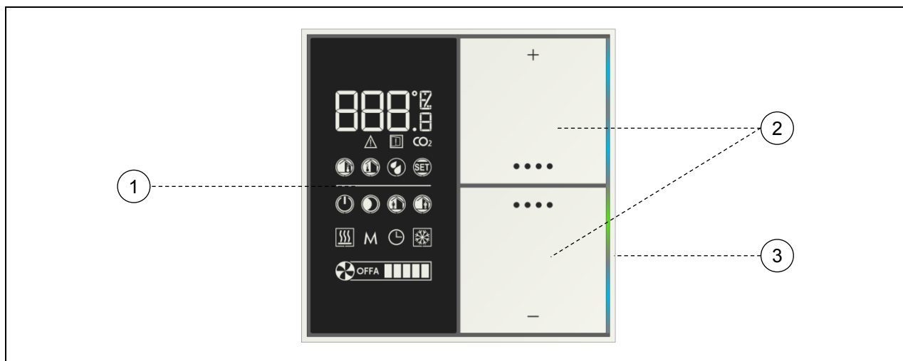
User interface: LC-display (1), rockers (2), LEDs (3) with lightguide
