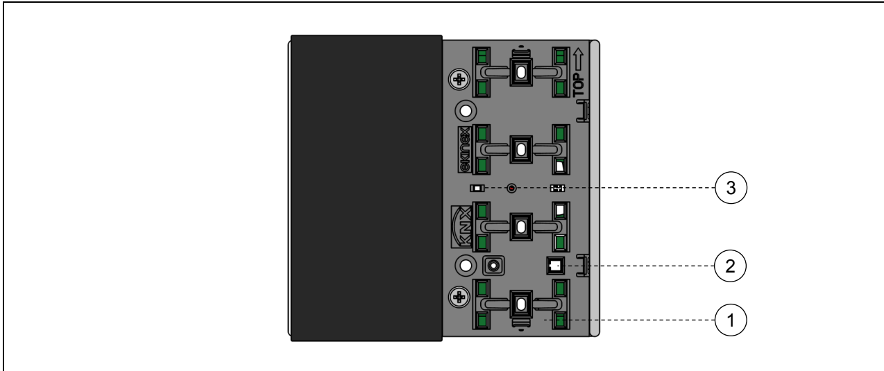
Position of the sensors: temperature (1), relative humidity (2) and brightness (3). The temperature sensor (not to be seen in the drawing) is located under the plastic half-shell for the rockers' mounting.
