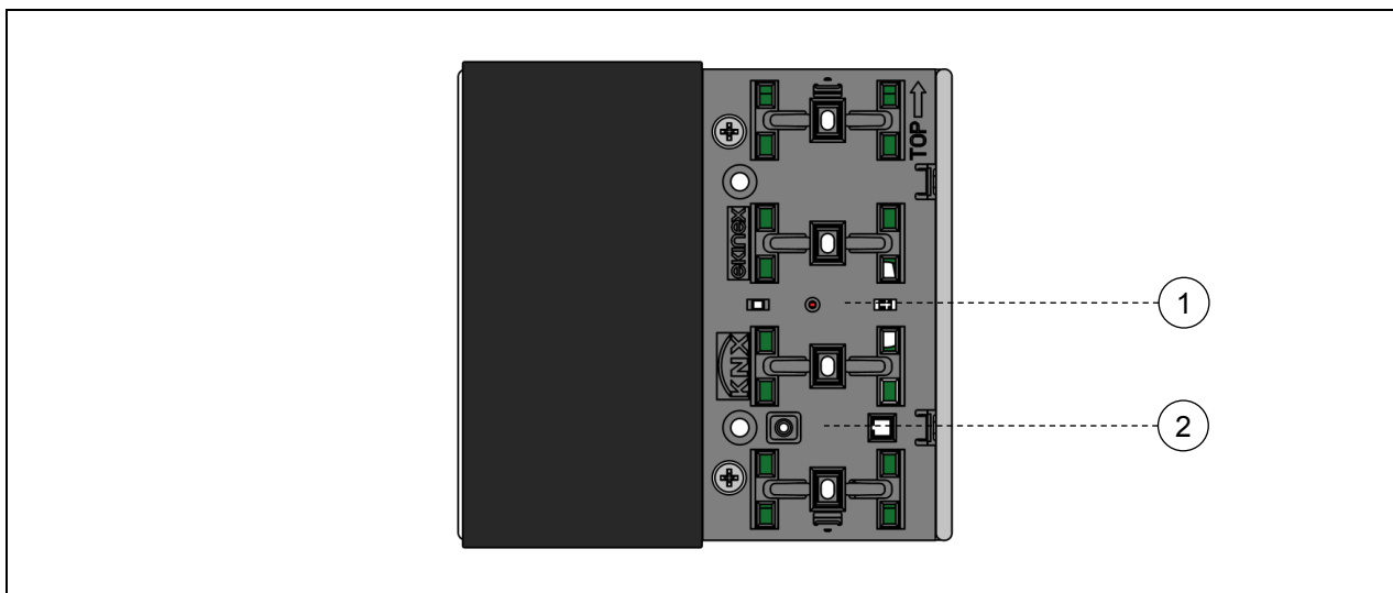
Device programming: led (1) and pushbutton (2)
