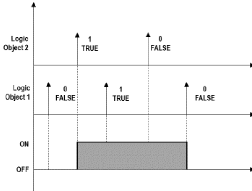
Figure 6 – Logic function OR
