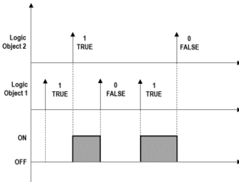
Figure 7 – Logic function AND
