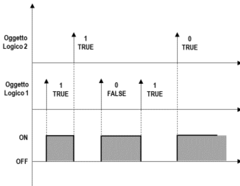
Figure 8 – Logic function Exclusive OR (XOR)
