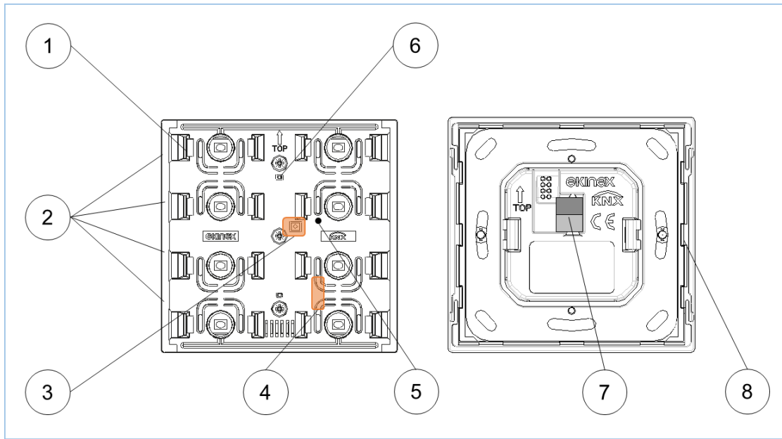
Figure 1 – Switching, display and connection elements
