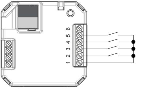
Connection of free-potential contacts
