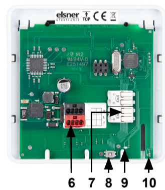
Fig. 4 Back view without mounting 6 KNX bus terminal +/- for connection when mounted on a socket 7 Spring-loaded terminals KNX bus for mounting directly on the wall 8 Programming button (recessed) for teaching device 9 Programming LED 10 Temperature sensor PRG key is accessible from below/outside when the device is mounted (see chapter Addressing the device).
