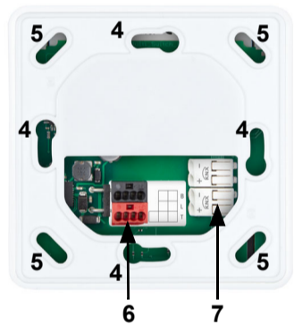
Fig. 3 Back view with mounting 4/5 Screw holes for different sockets. Fastening with 2 screws is sufficient. For wall mounting, use a fixing material suitable for the ground! 6 KNX bus terminal +/- for connection when mounted on a socket 7 Spring-loaded terminals KNX bus for mounting directly on the wall
