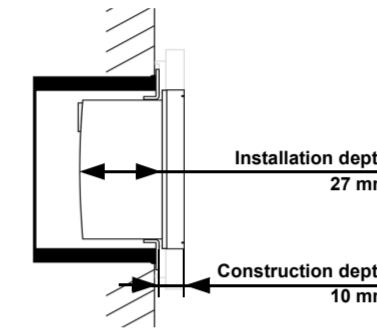
Fig. 2: Sectional drawing. The Cala KNX T 201/202 Sunblind push button fits in a standard connector socket (Ø 60 mm, depth 42 mm). The frame is not included in the delivery!
