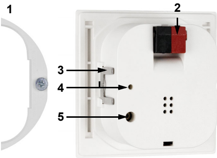
Fig. 4 Rear 1 Mounting adapter 2 KNX terminal BUS +/- 3 Catches 4 Programming LED (recessed) 5 Programming LED (recessed) for teaching the device
