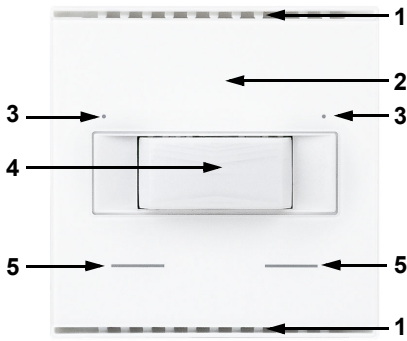
Fig. 3 Front 1 Ventilation slots (top and bottom) 2 Position of the brightness sensor 3 LEDs 4 Presence sensor 5 Touch buttons
