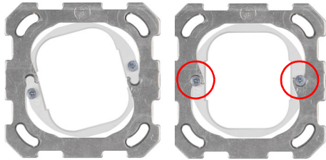
Fig. 5 Hook the mounting adapter into the mounting plate of the switch system and tighten the screws.
