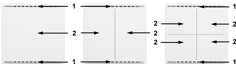
Fig. 2: Front
