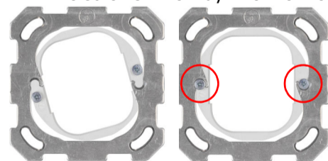
Fig. 4 Hook the mounting adapter into the mounting plate of the switch system and tighten the screws.
