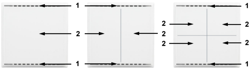
Fig. 2: Front 1 Ventilation slit (top and bottom) 2 Touch areas with LEDs
