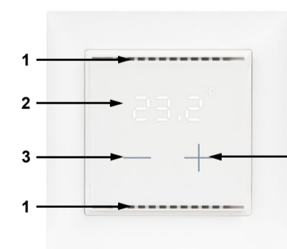
Fig. 1: Front 1 Ventilation slit (top and bottom) 2 Temperatur display 3 Touch area - 4 Touch area +
