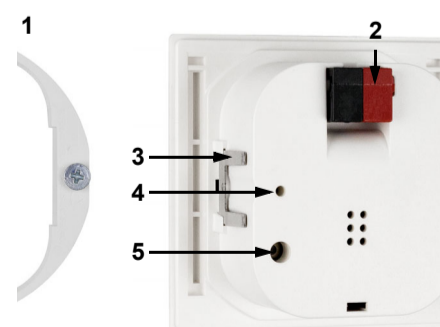
Fig. 2: Rear 1 Mounting adapter 2 KNX terminal BUS +/- 3 Catches 4 Programming LED (recessed) 5 Programming LED (recessed) for teaching the device
