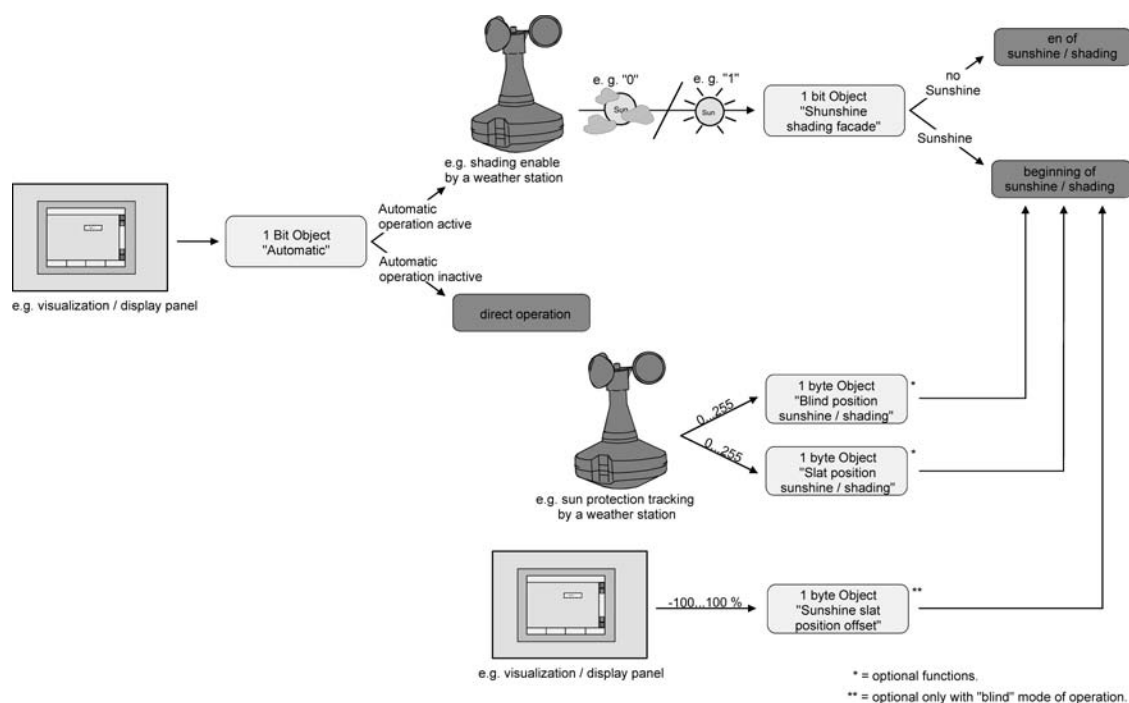
picture 22: Schematic diagram illustrating the extended sun protection configuration (for reasons of simplicity without disabling functions)
