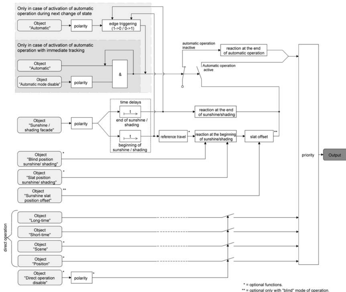
picture 23: Function diagram illustrating the extended sun protection
