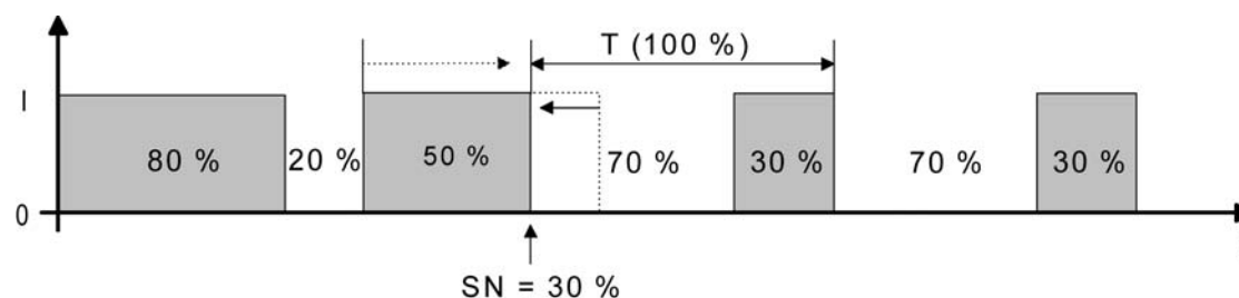
picture 42: Command value change, e.g. from 80 % to 30 % during the opening phase of the valve (opening phase too long)
