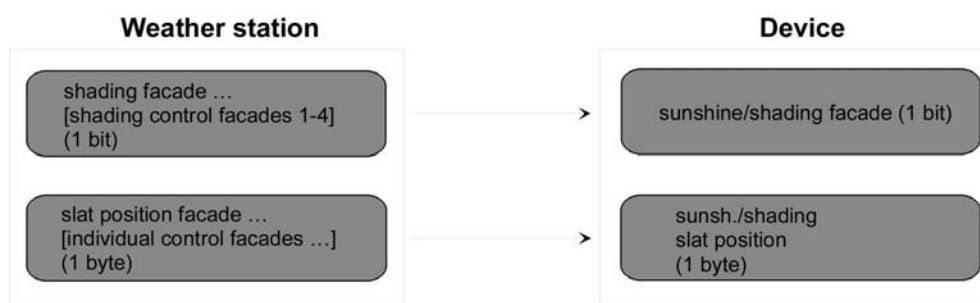
picture 27: Programming of the communication objects for application example III
