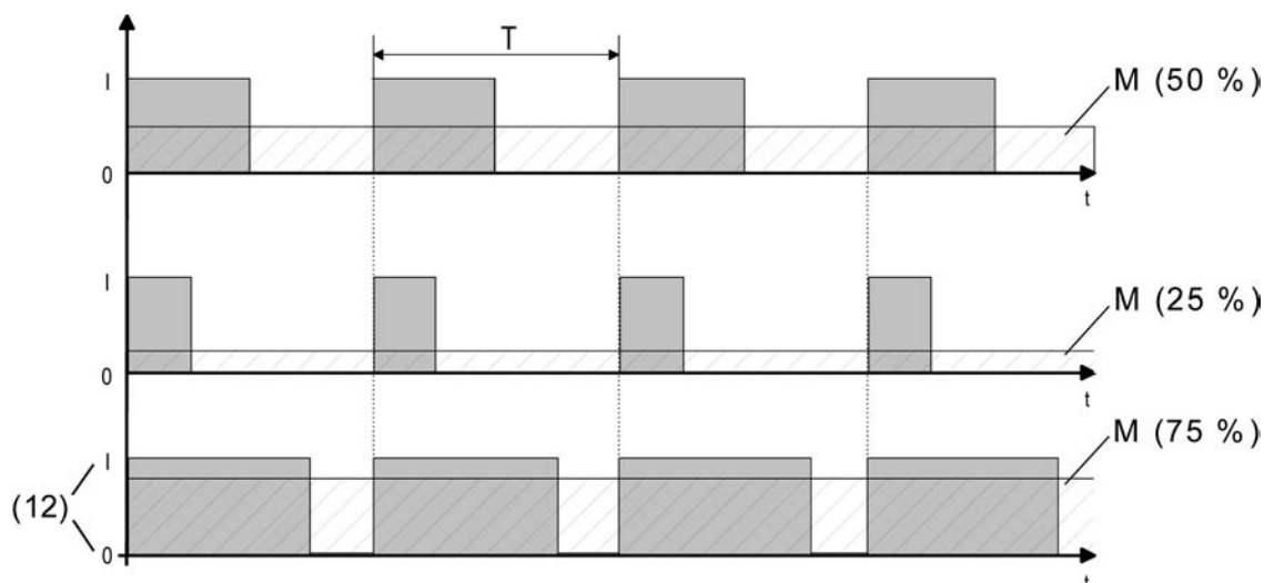
picture 39: Pulse width modulation of a valve output signal
