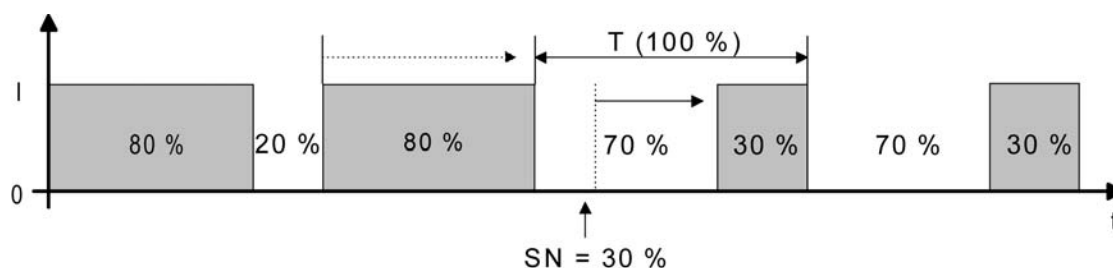
picture 41: Command value change, e.g. from 80 % to 30 % during the closing phase of the valve
