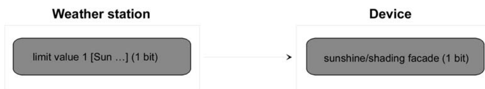
picture 25: Programming of the communication objects for application example I.
