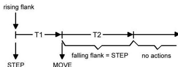
picture 6: Operating concept "Short - long - short" when inputs 1 and 2 have an internal impact
