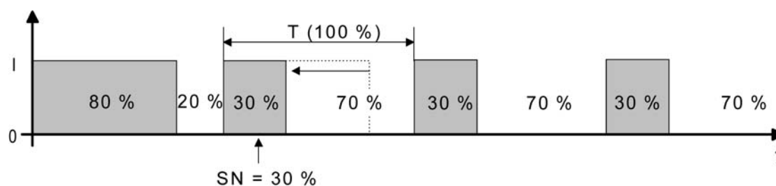
picture 40: Command value change, e.g. from 80 % to 30 % during the opening phase of the valve
