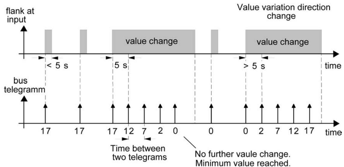
picture 9: Example to change the value for dimming value encoder
