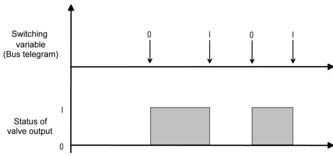
picture 35: Conversion of a switching command value to an output signal with deenergised, opened valve drives (example)
