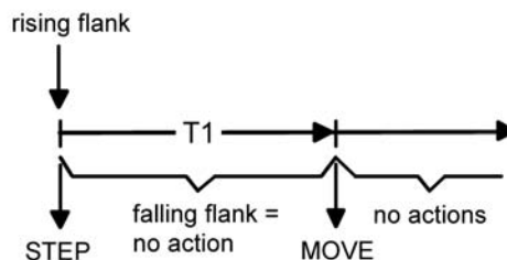
picture 8: Operation concept "long – short"
