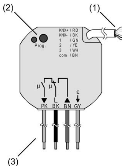
picture 1: Device components
