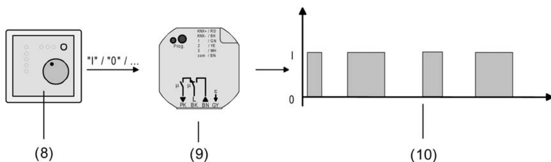
picture 37: Command value principle for switching command value
