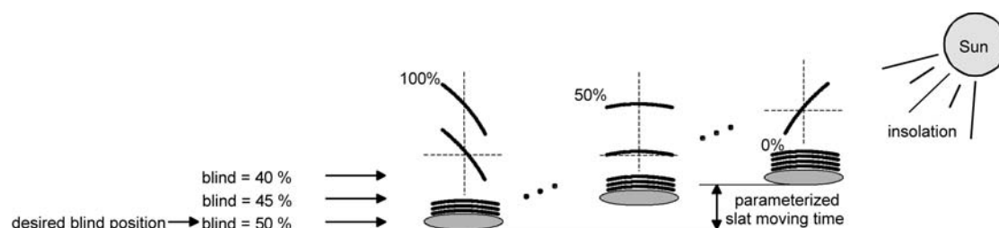
picture 15: Example of slat positioning affecting the position of the Venetian blind (typical of slat type 1; analogous reaction for type 2)
