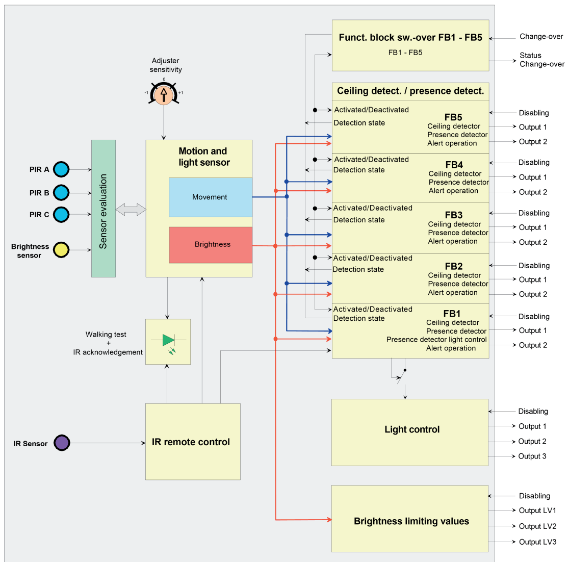
Figure 15: Block diagram of all device functions
