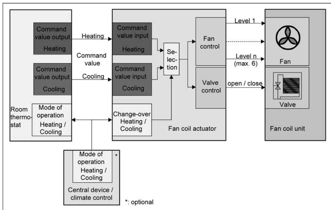
picture 13: Functional diagram for "2-pipe heating/cooling via change-over object"
