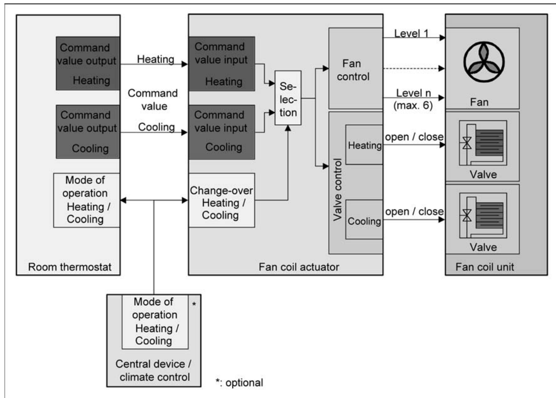
picture 14: Functional diagram for "4-pipe heating/cooling via change-over object"
