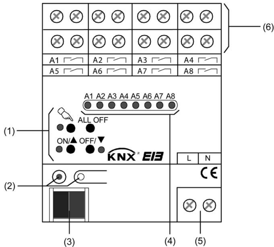
picture 1: Device components
