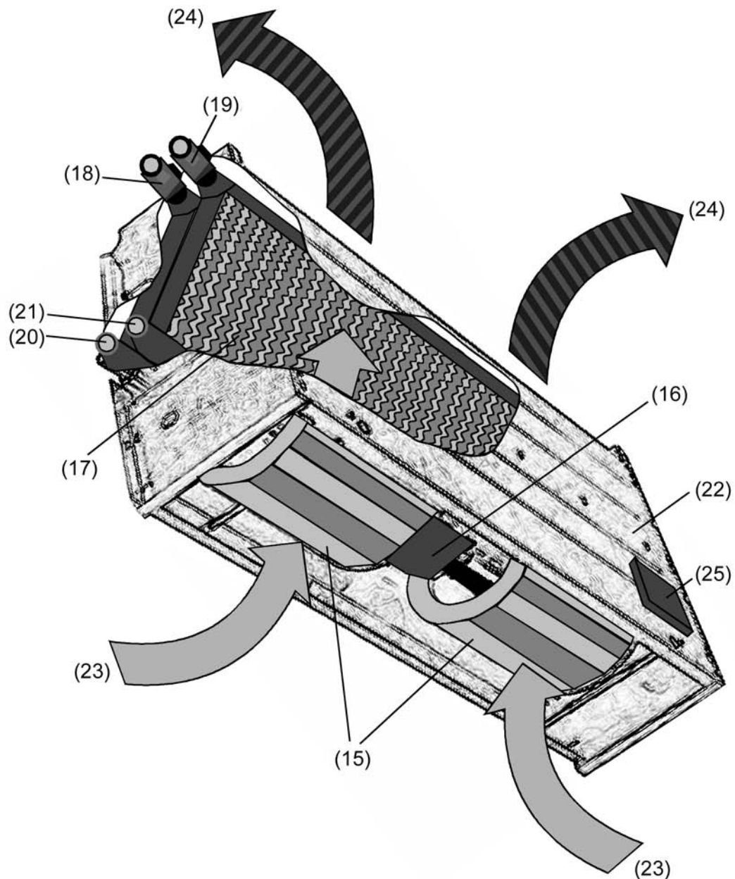
picture 7: The fan coil principle (example based on a 4-pipe fan coil unit with upright design)
