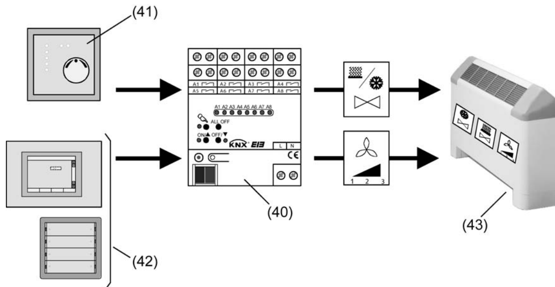
picture 28: Principle of manual fan control
