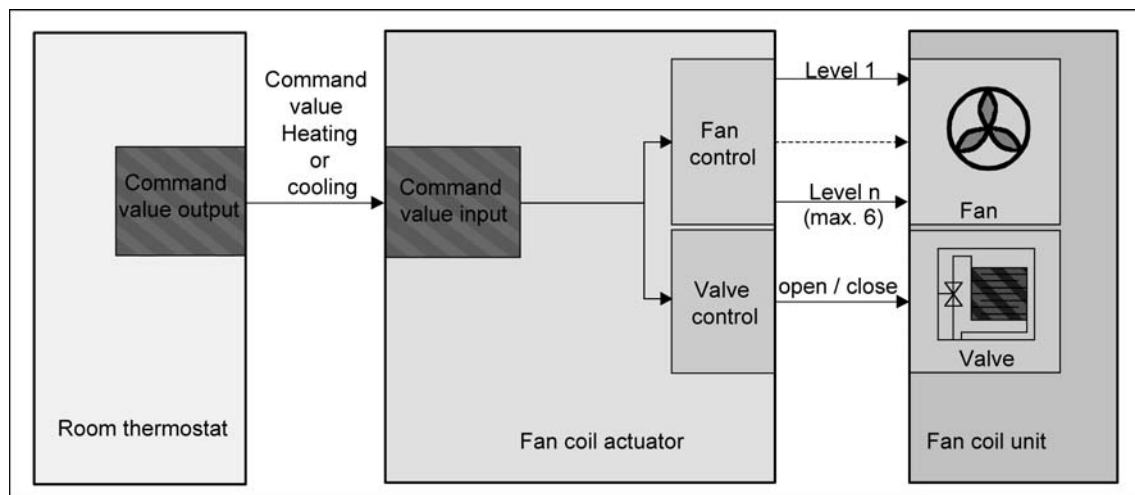
picture 12: Functional diagram for "2-pipe only heating" and "2-pipe only cooling"
