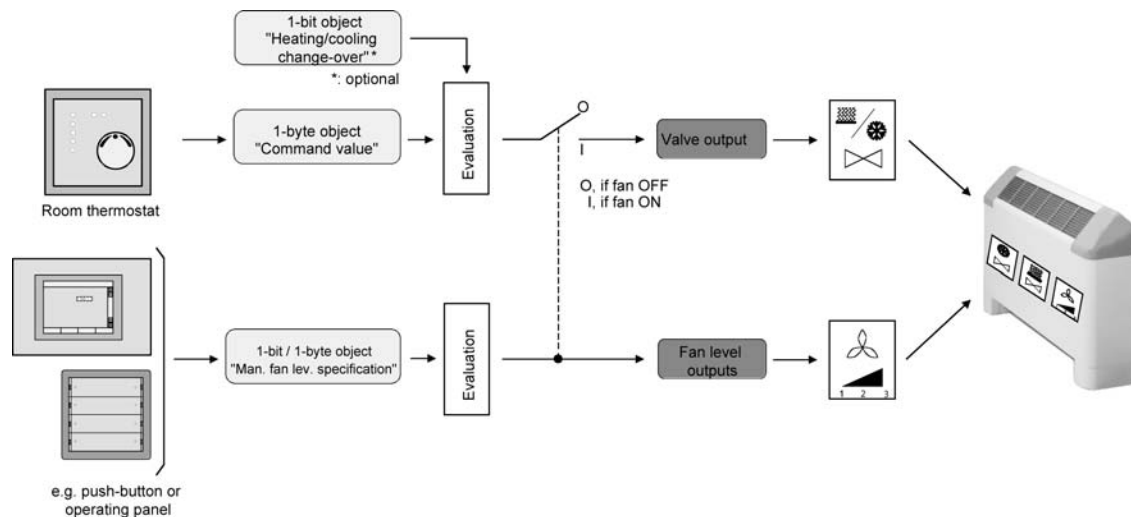
picture 29: Schematic diagram for manual fan control independent of active heating / cooling (simplified depiction)
