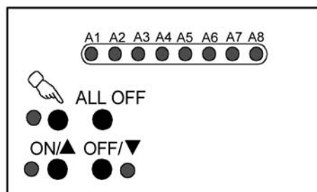
picture 16: Elements for manual control on the front panel of the device
