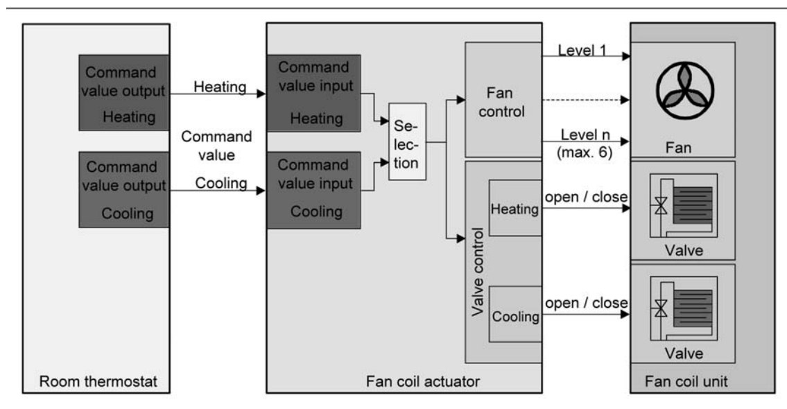
picture 15: Functional diagram "4-pipe heating/cooling via command value specification"
