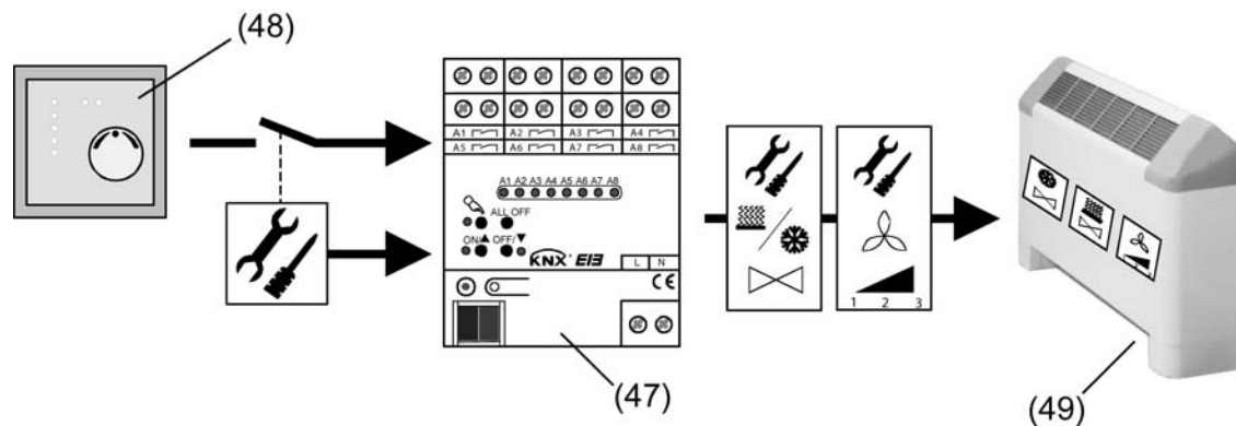
picture 32: Principle of the disabling function - example showing a maintenance interlock
