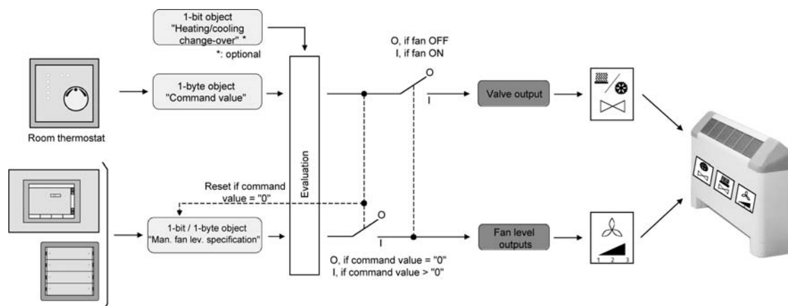
picture 30: Schematic diagram for manual fan control depending on active heating / cooling (simplified depiction)
