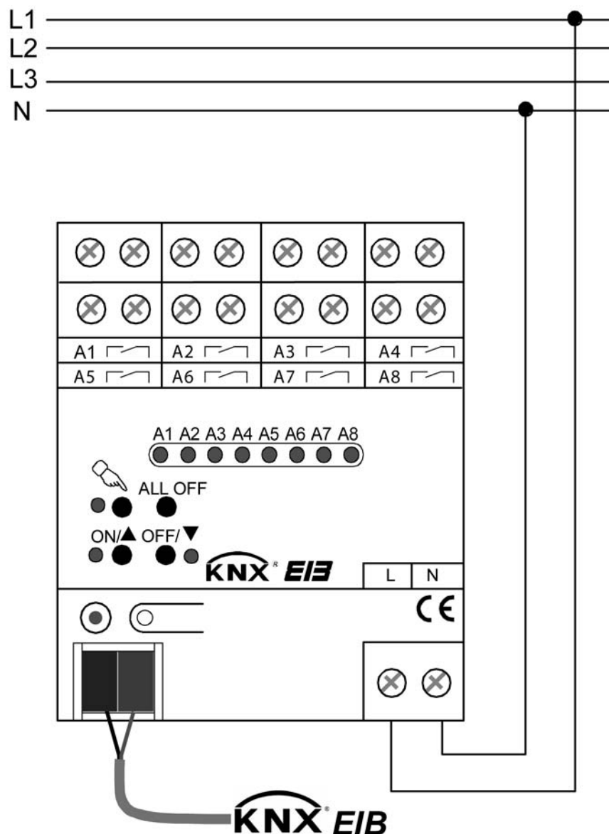
picture 2: Electrical connection of mains voltage
