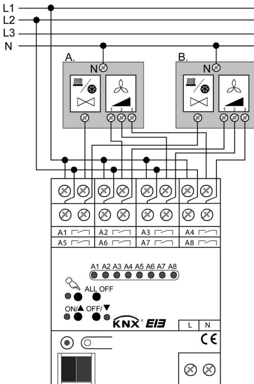
picture 4: Electrical connection for fan coil units (A. + B.) in 2-channel operation (connection example)
