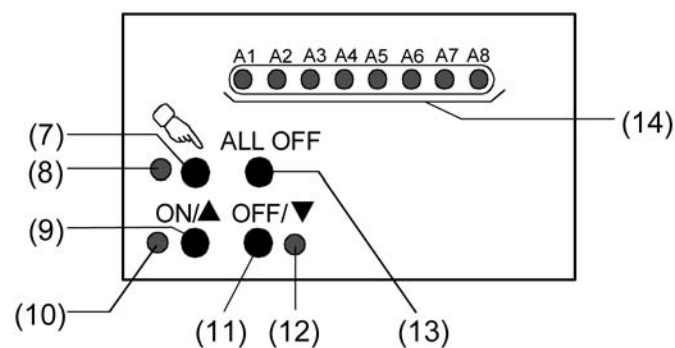
picture 6: Controls and indicators for manual control
