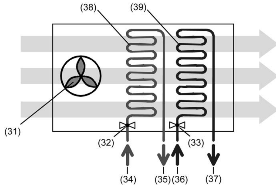
picture 9: The 4-pipe system
