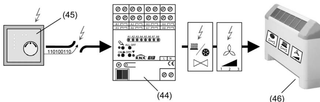
picture 31: Principle of cyclical command value monitoring in the event of a fault (e.g. open circuit)
