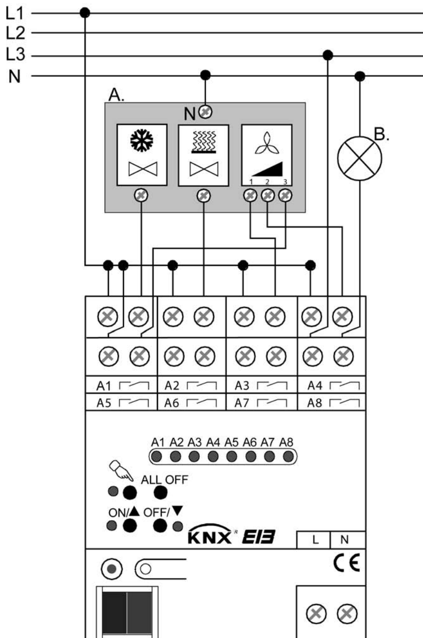
picture 3: Electrical connection for fan coil unit (A.) in 1-channel operation with additional simple switching load (B.) (connection example)
