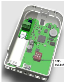
Fig. Built-in DIP-switch block
