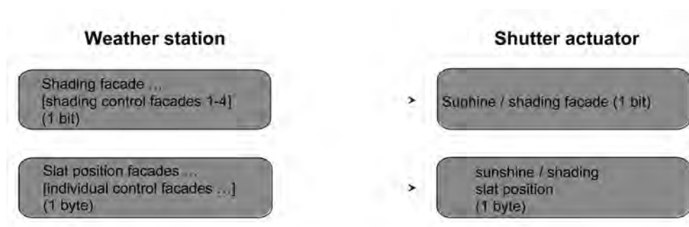
Figure 42: Programming of the communication objects for application example III
