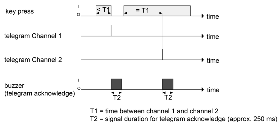
Figure 10: Example of operation concept "Channel 1 or Channel 2"
