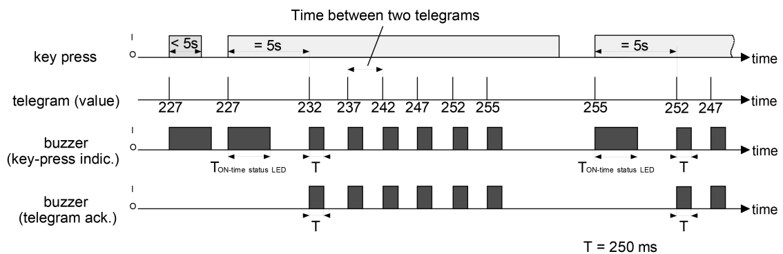
Figure 8: Example of value adjustment without value range overflow
