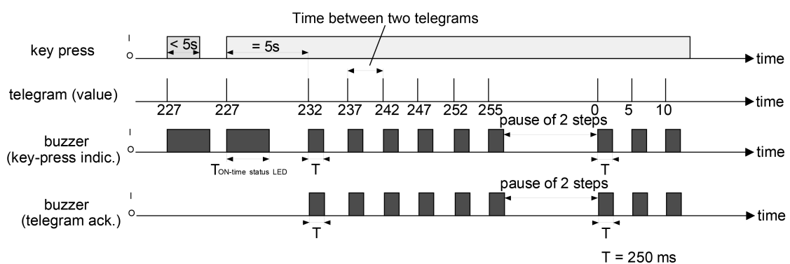
Figure 9: Example of value adjustment with value range overflow
