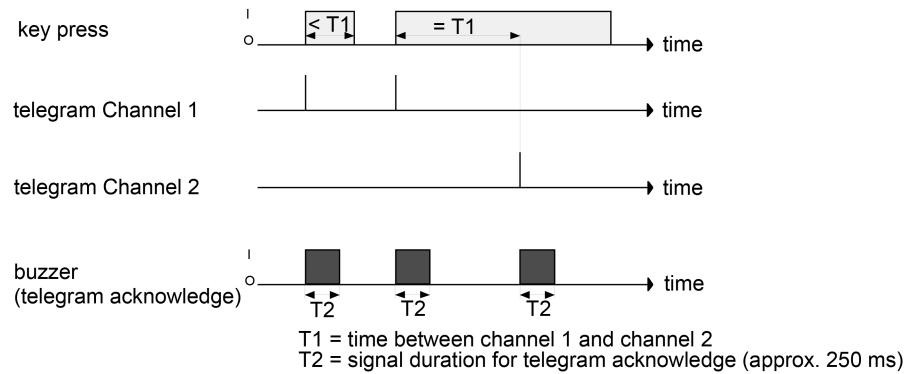
Figure 11: Example for operation concept "Channel 1 and channel 2"
