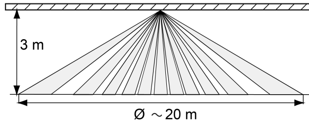
Figure 2: Diameter of the detection area at installation height 3 m
