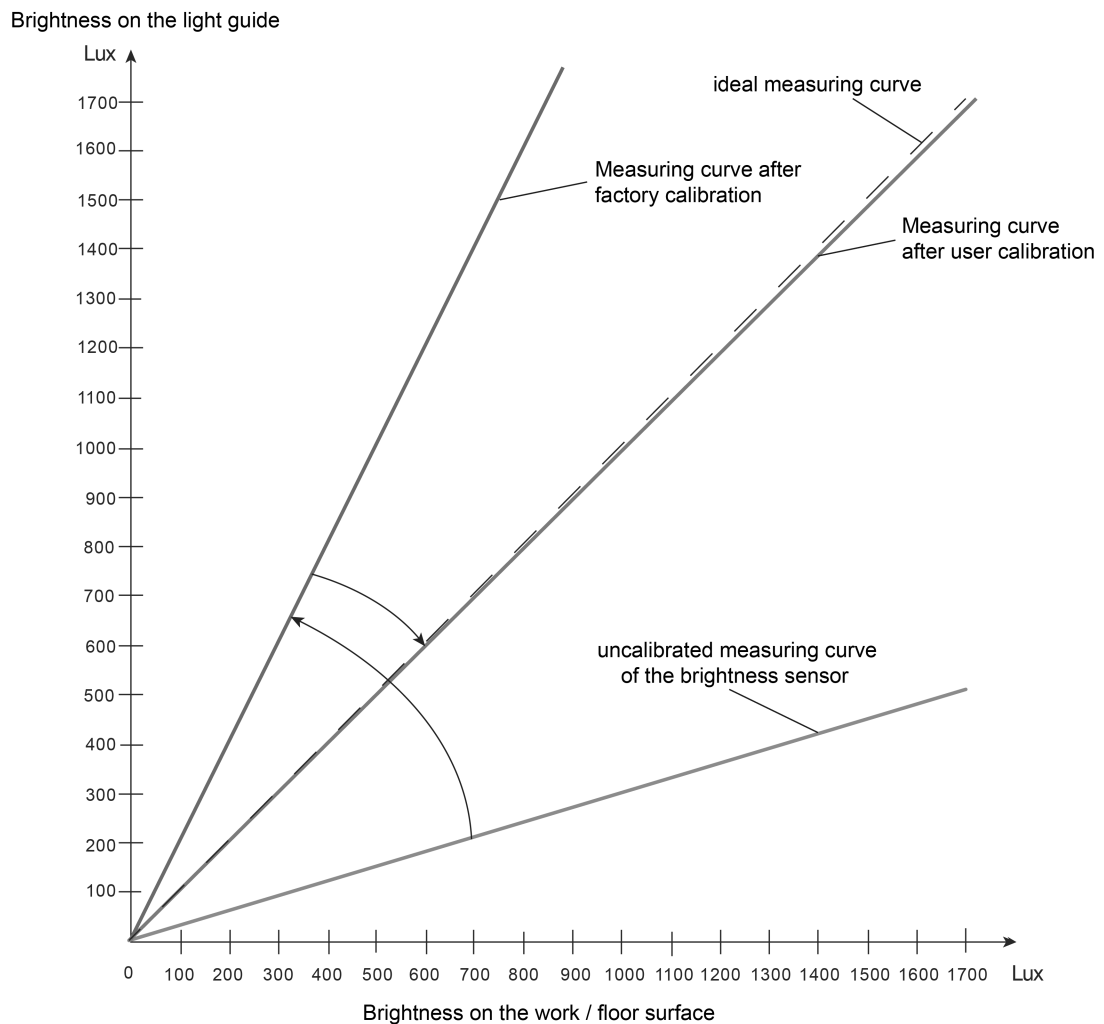
Figure 14: Correction of the determined brightness on the work / floor surface by means of user calibration e.g. reflection coefficient 0.5 corresponds to surface finish (light floor covering)
