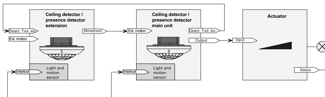
Figure 28: Application example with twilight level evaluation in the main unit and extensions Universal solution for all data formats
