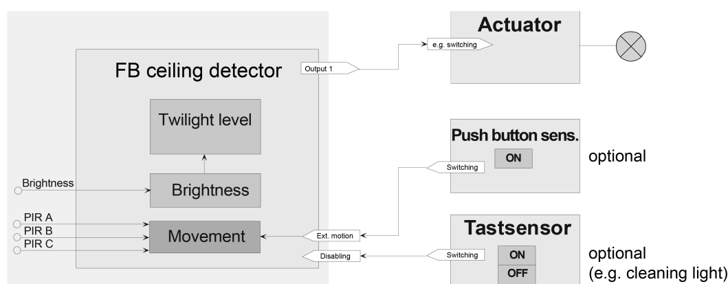
Figure 15: Application example of the application ceiling detector
