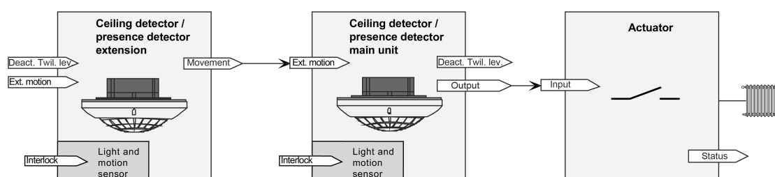
Figure 30: Application example without twilight level evaluation in the main unit and extensions
