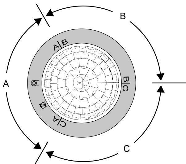
Figure 10: Arrangement of the PIR sectors A, B and C
