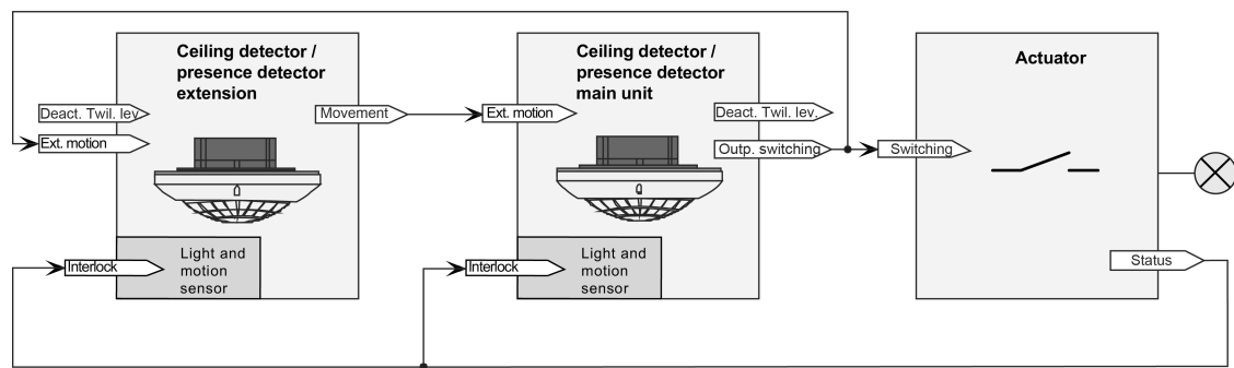
Figure 29: Application example with twilight level evaluation in the main unit and extensions for output function "Staircase function"
