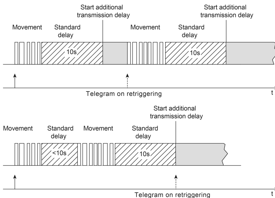
Figure 33: Triggering of a telegram when retriggering
