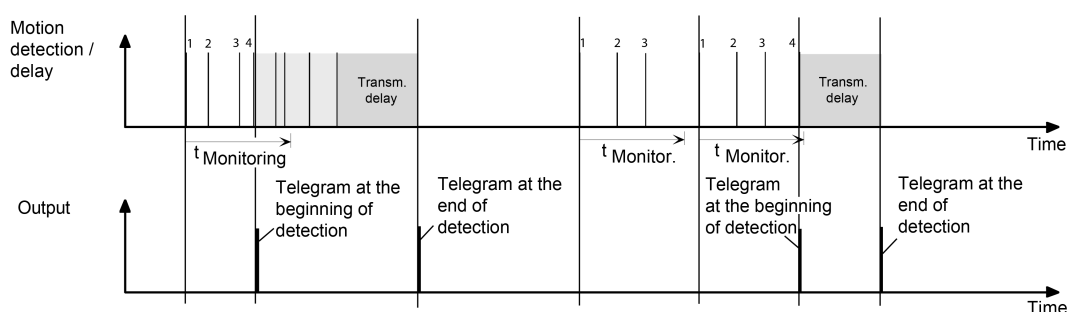
Figure 36: Motion evaluation with the detector
