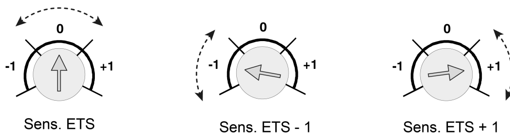
Figure 8: Adjustment ranges of the adjuster "Sens." on the device (-1 <-> 0 <-> +1)
