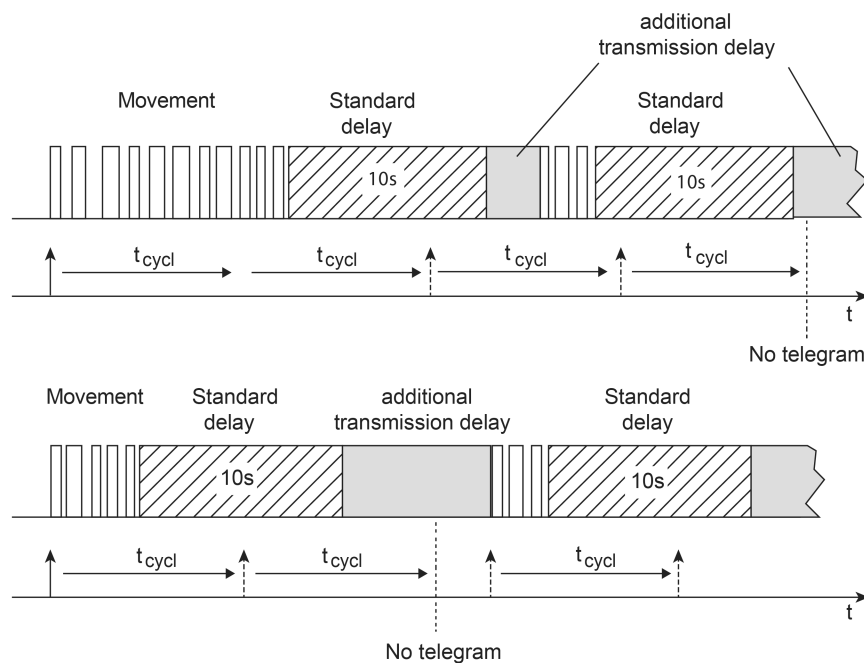
Figure 32: Cyclical transmission during a motion detection
