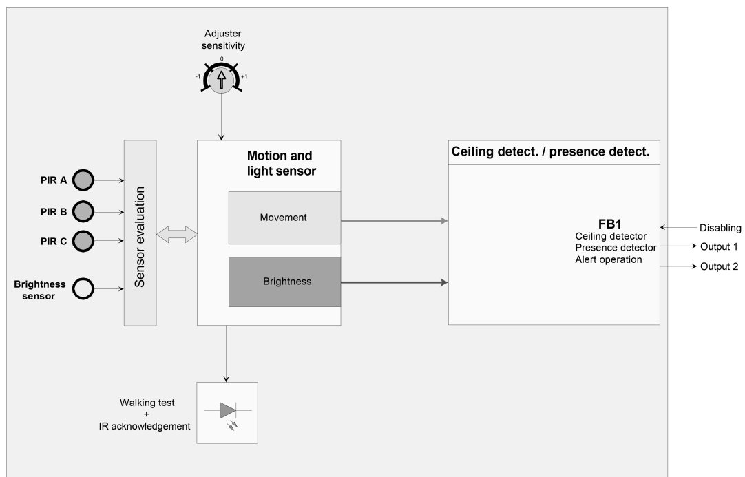
Figure 9: Block diagram of all device functions
