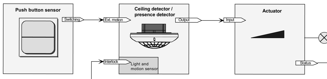
Figure 24: Application example of single device with external motion detection
