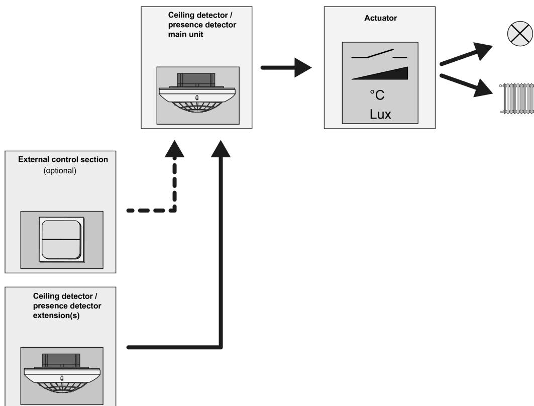
Figure 21: Application type "Main unit"
