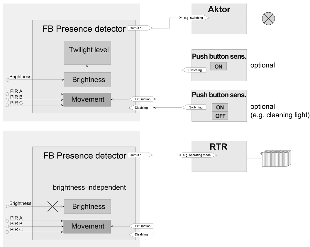
Figure 17: Application examples of the application presence detector
