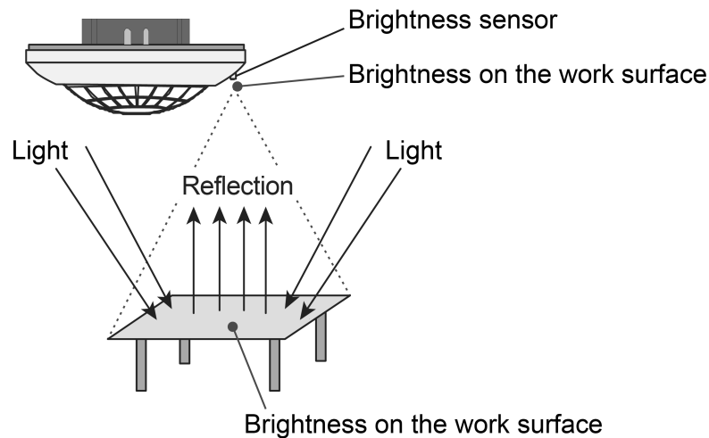
Figure 12: Brightness determination by measuring reflected mixed light composed of artificial light and daylight
