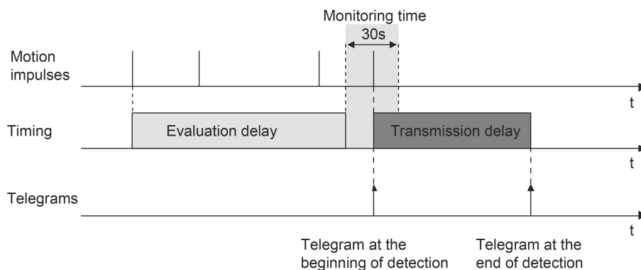
Figure 34: Evaluation delay with ongoing motion
