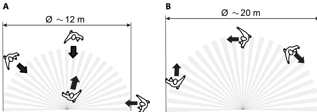
Figure 3: Detection range depending on the direction of movement at installation height of 3 m
