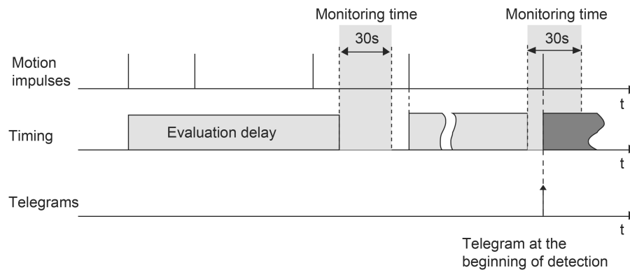
Figure 35: Evaluation delay with only brief motion
