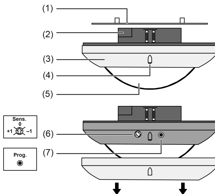
Figure 1: Device components
