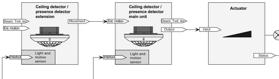
Figure 25: Application example of main unit and extension without twilight level evaluation
