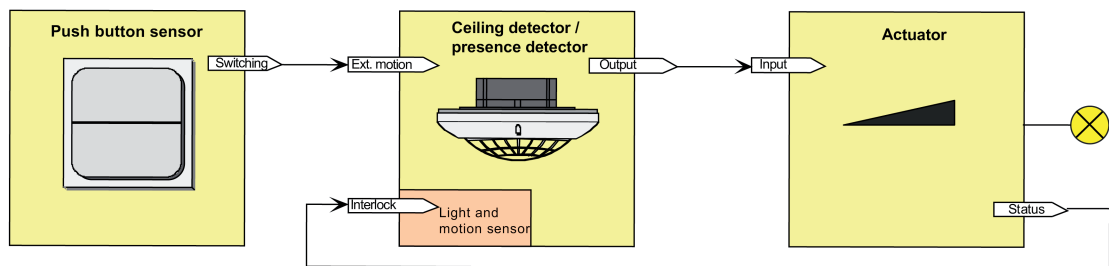
Figure 26: Application example of single device with external motion detection
