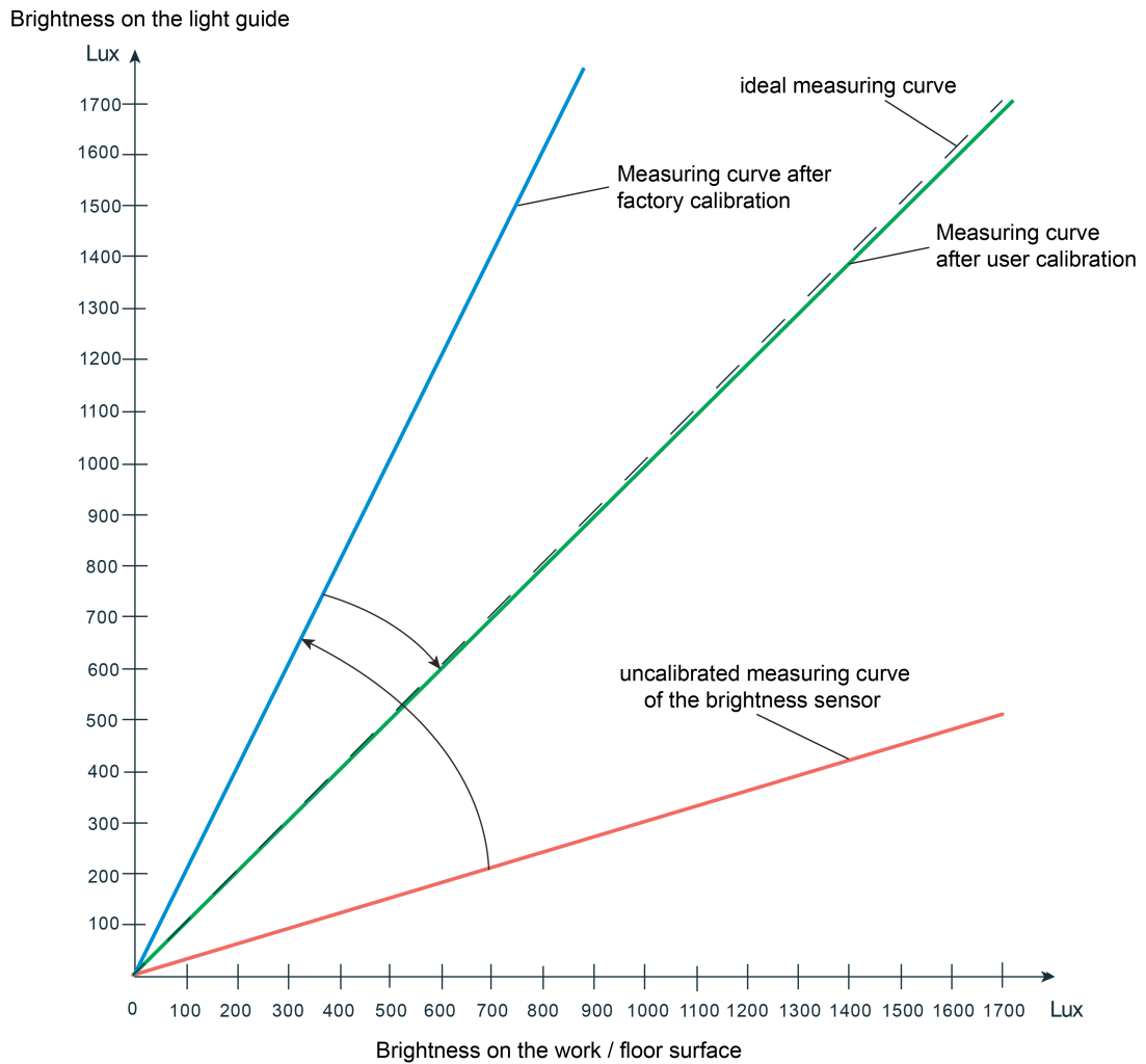
Figure 15: Correction of the determined brightness on the work / floor surface by means of user calibration e.g. reflection coefficient 0.5 corresponds to surface finish (light floor covering)
