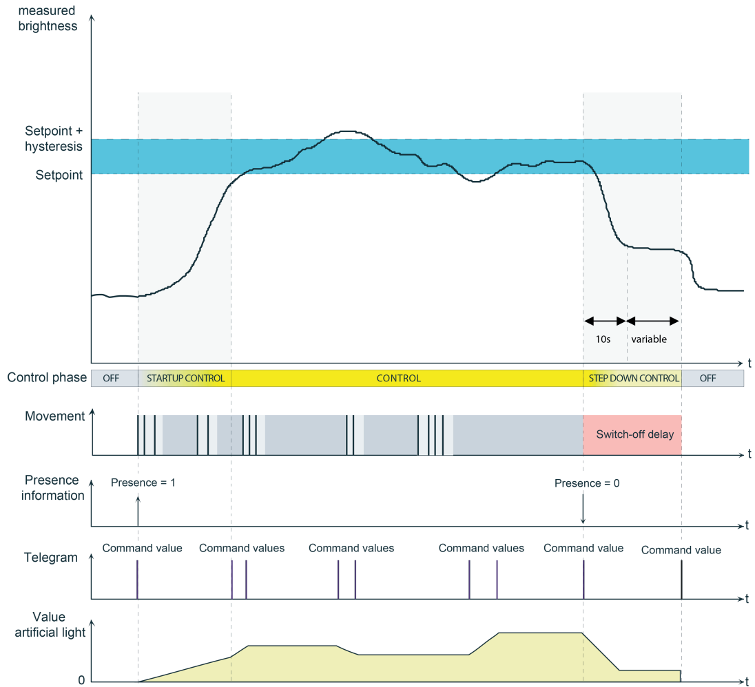
Figure 40: Example of a control process with all control phases
