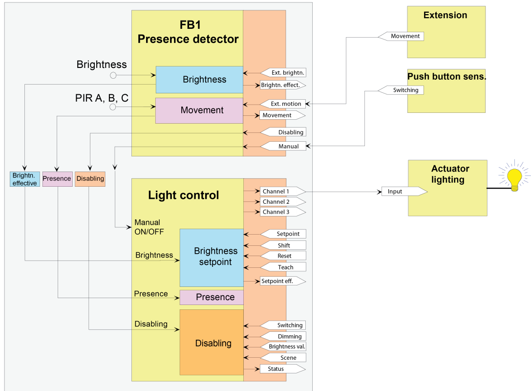
Figure 42: Application example for light control in combination with function block 1
