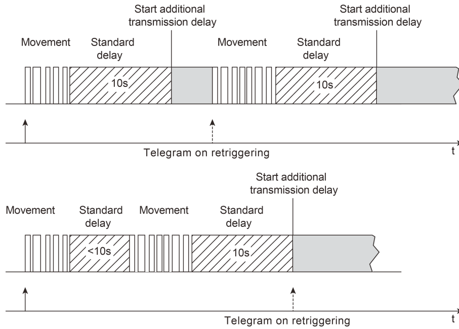
Figure 35: Triggering of a telegram when retriggering
