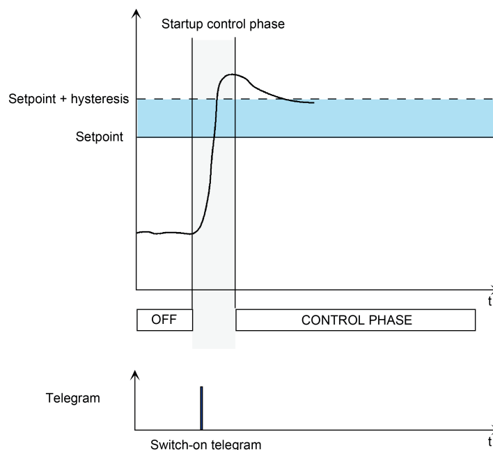
Figure 49: Startup control behaviour with switching telegram (1-bit)
