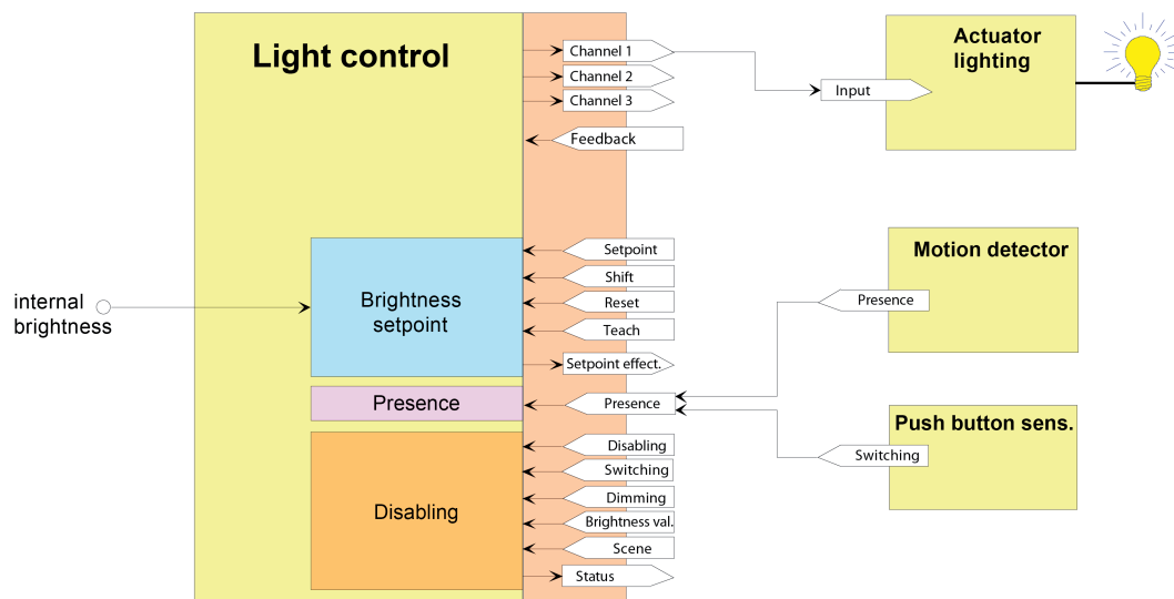
Figure 41: Application example for light control in autonomous operation
