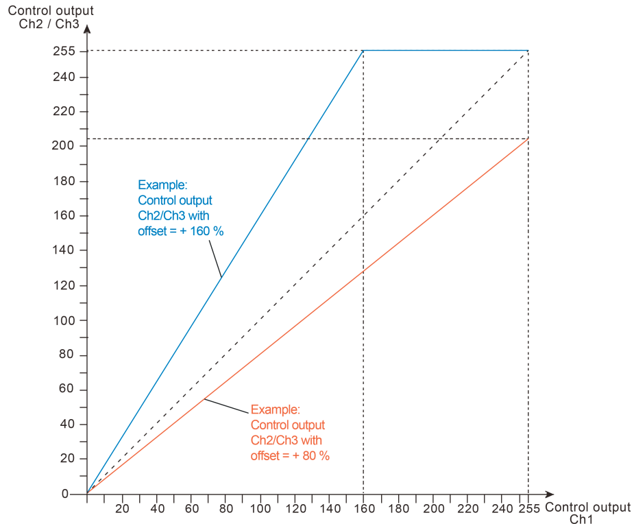
Figure 47: Control outputs of channels 2 or 3 dependent on the control output of channel 1 Method 2: Offset increasing with increasing control output
