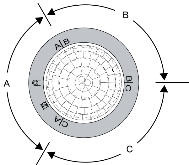
Figure 11: Arrangement of the PIR sectors A, B and C
