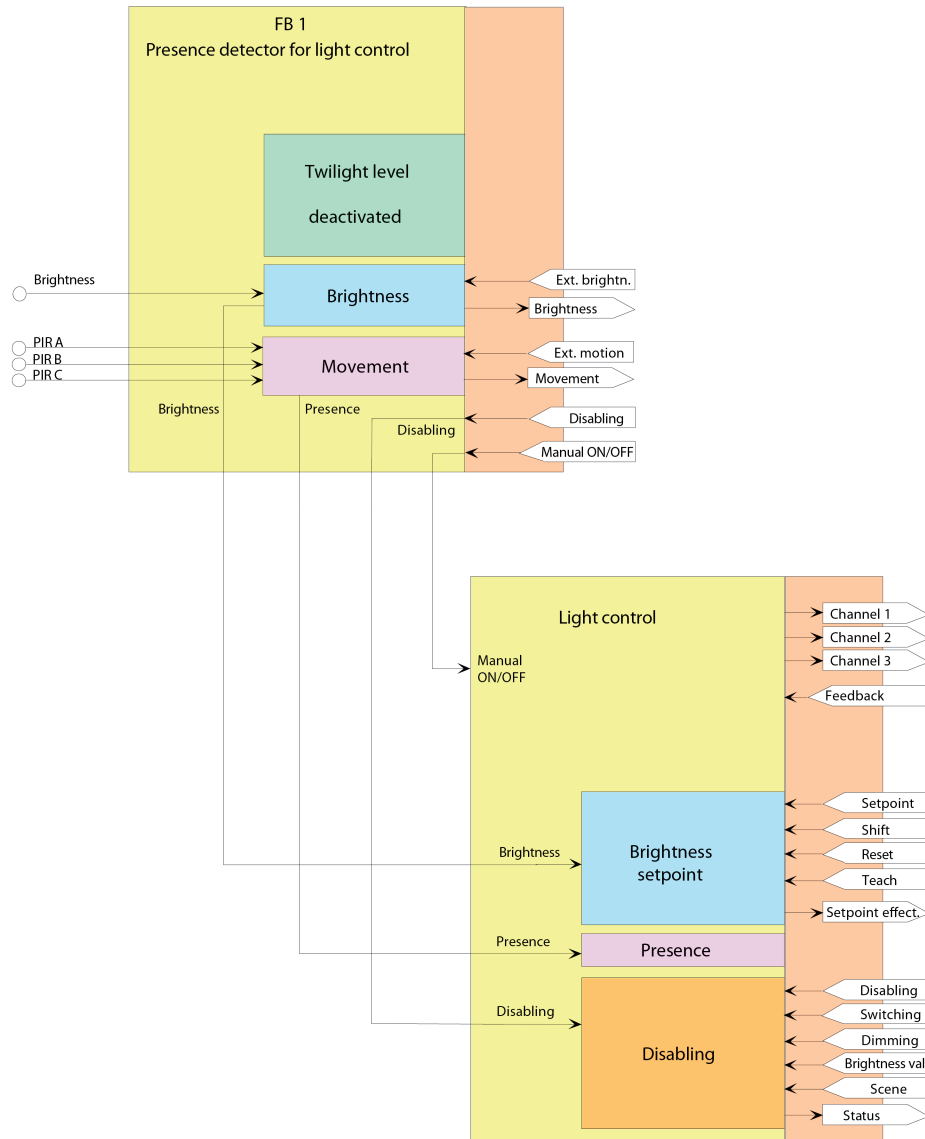
Figure 21: Function elements of the application presence detector with light control
