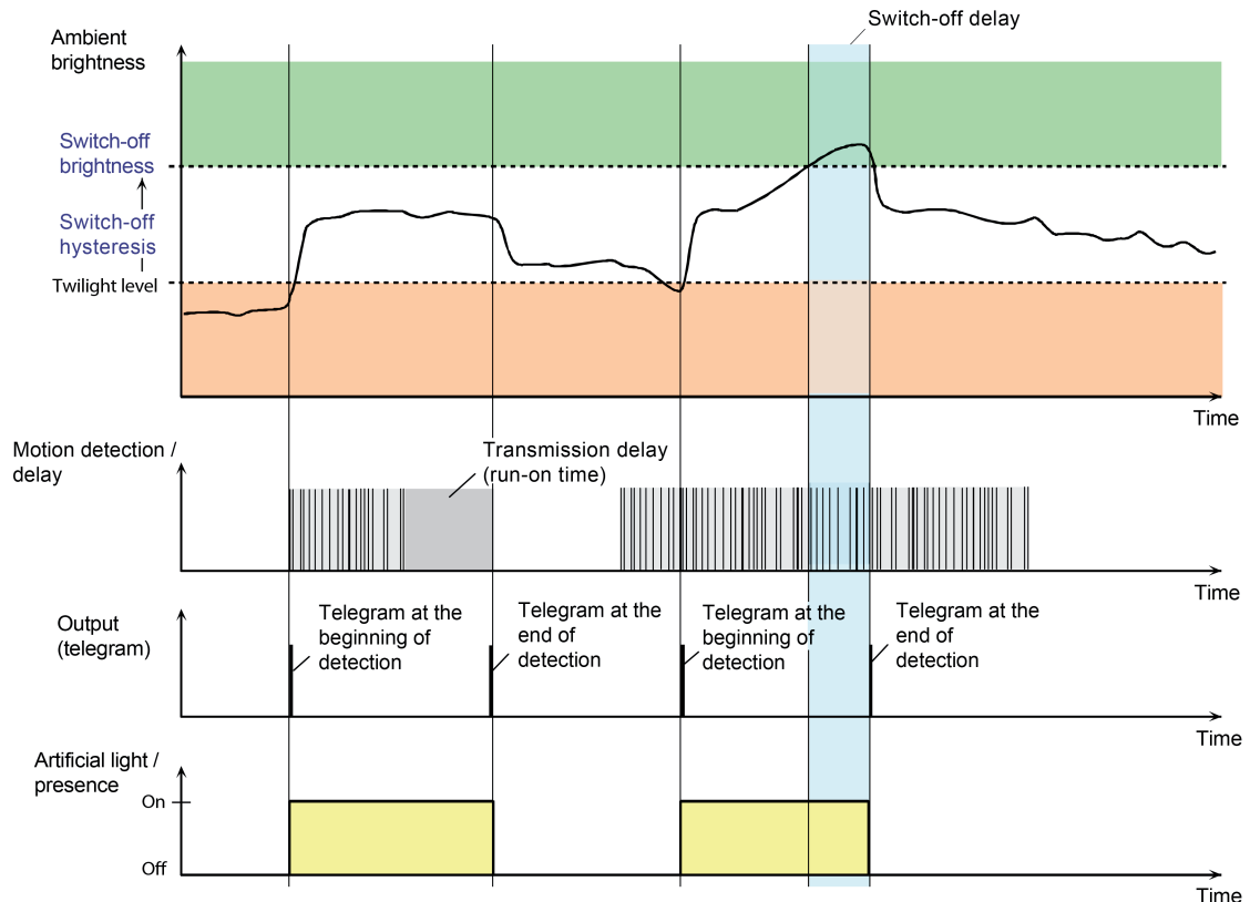
Figure 19: Brightness and motion evaluation with the presence detector
