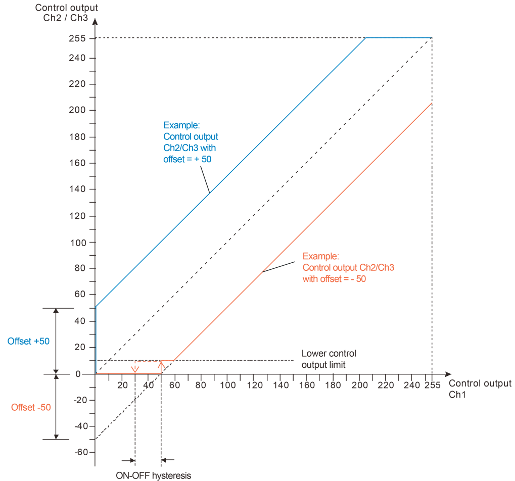
Figure 46: Control outputs of channels 2 or 3 dependent on the control output of channel 1 Method 1: Fixed offset with increasing control output
