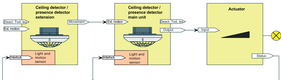
Figure 28: Application example of main unit and extension with twilight level evaluation in the main unit
