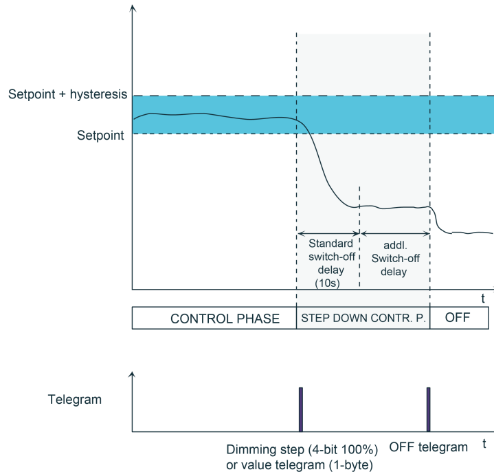
Figure 56: Step down control behaviour with waiting time
