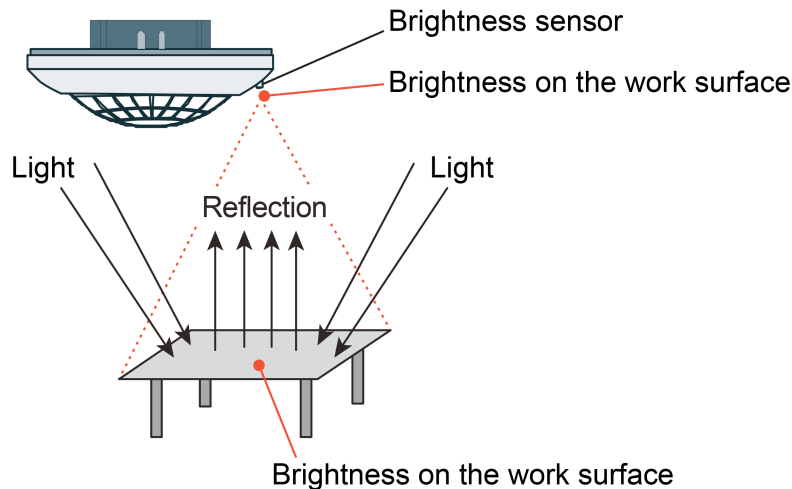
Figure 13: Brightness determination by measuring reflected mixed light composed of artificial light and daylight
