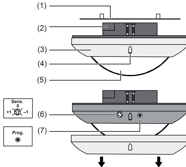
Figure 1: Device components
