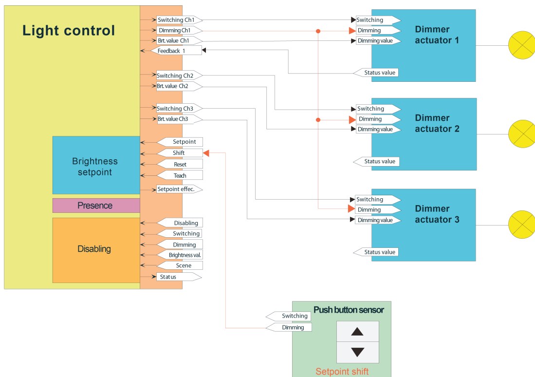
Figure 45: Application example for the setpoint shift with 3 lighting channels
