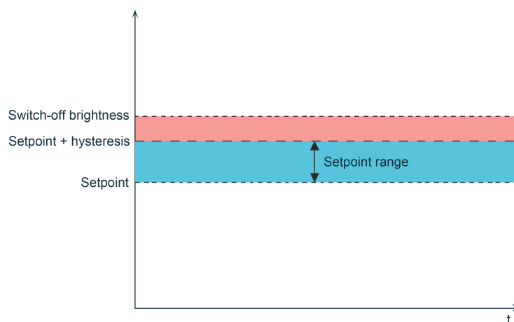
Figure 53: The switch-off brightness results relatively from the setpoint and hysteresis value of the setpoint
