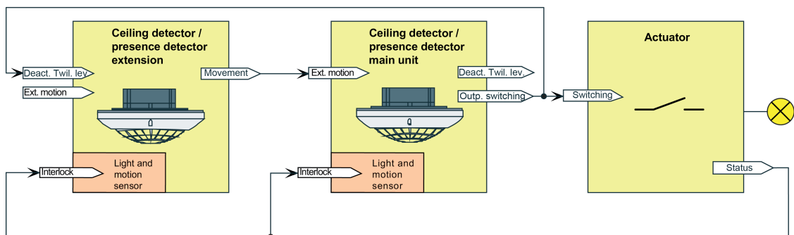
Figure 29: Application example with twilight level evaluation in the main unit and extensions for the data format "Switching"
