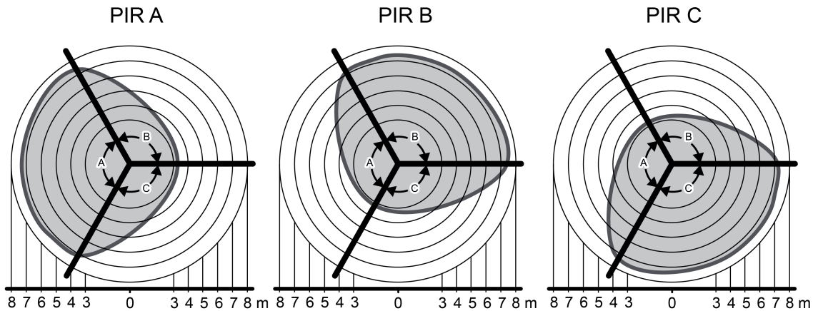
Figure 5: Detection field with PIR sectors A, B and C at an installation height of 2.50 m
