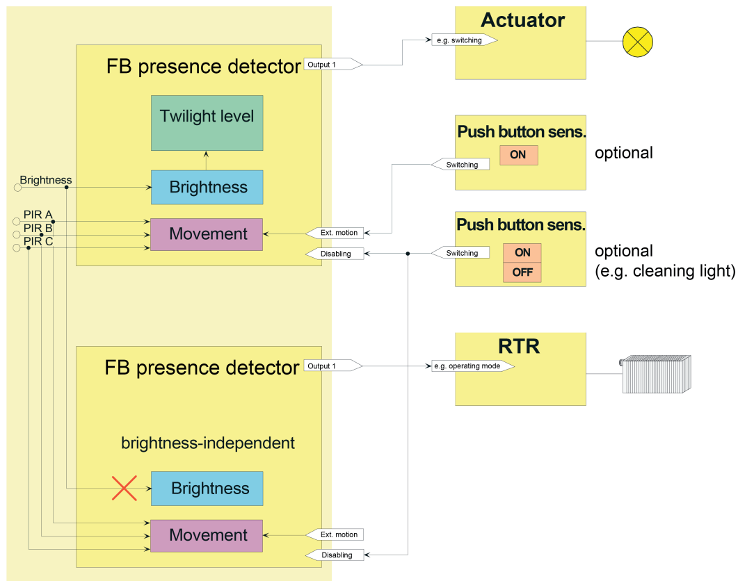
Figure 18: Application example of the application presence detector
