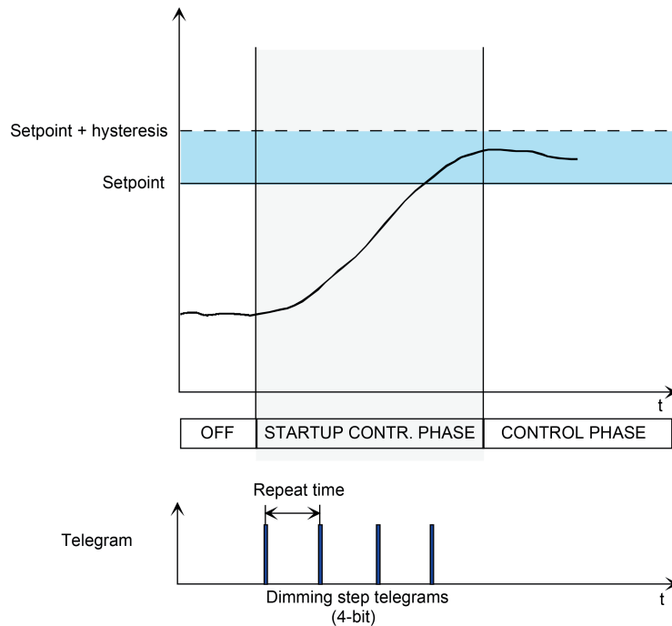
Figure 50: Startup control behaviour with relative dimming step telegrams (4-bit)
