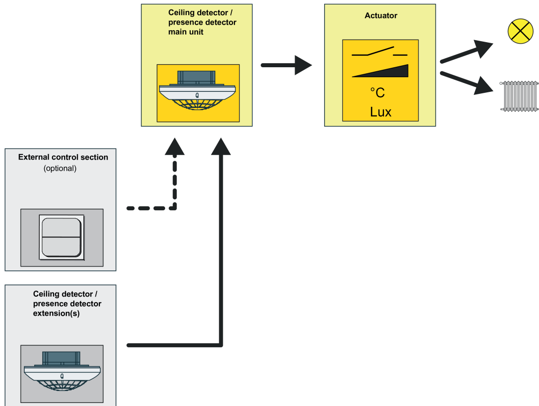
Figure 23: Application type "Main unit"
