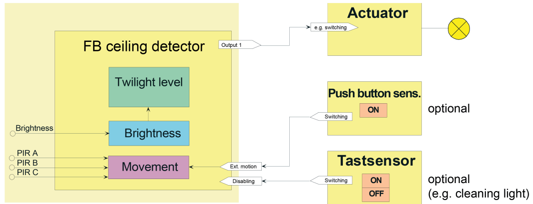
Figure 16: Application example of the application ceiling detector
