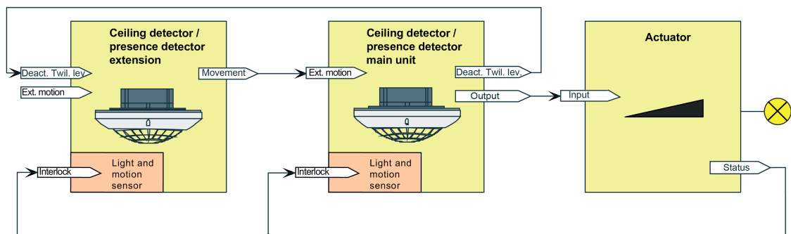
Figure 30: Application example with twilight level evaluation in the main unit and extensions Universal solution for all data formats
