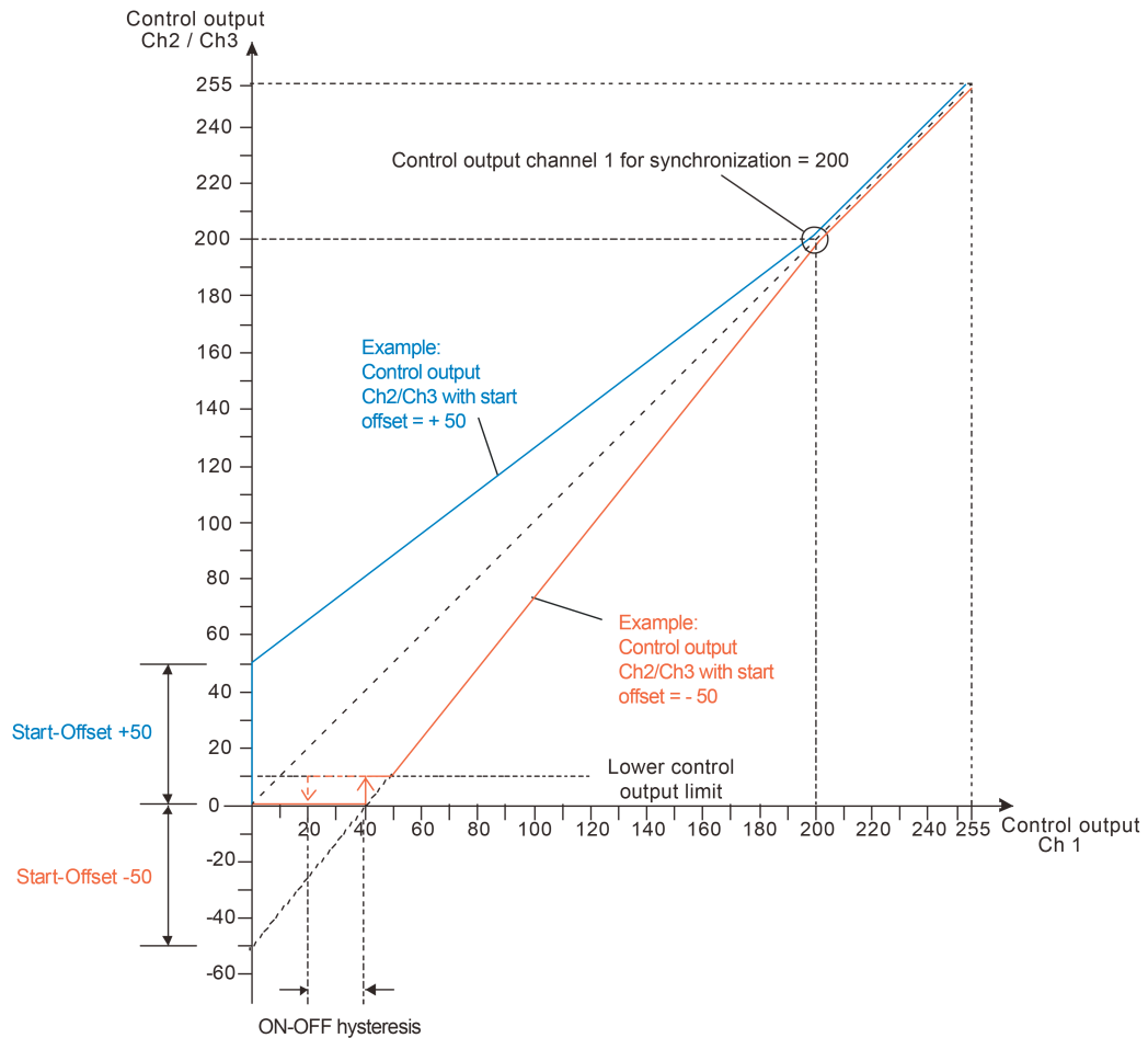
Figure 48: Control outputs of channels 2 or 3 dependent on the control output of channel 1 Method 3: Offset decreasing with increasing control output
