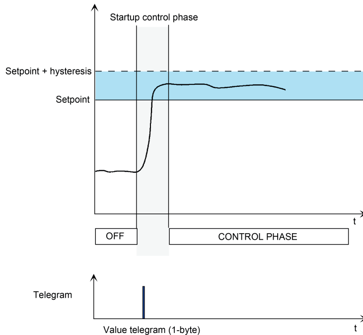
Figure 52: Startup control behaviour with adaptive control output presetting (1-byte)
