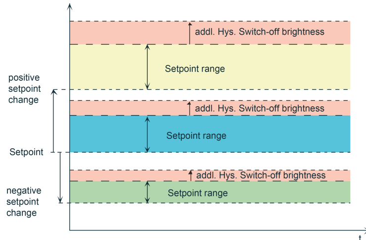
Figure 55: Dependency of the additional hysteresis for the switch-off brightness during a setpoint shift
