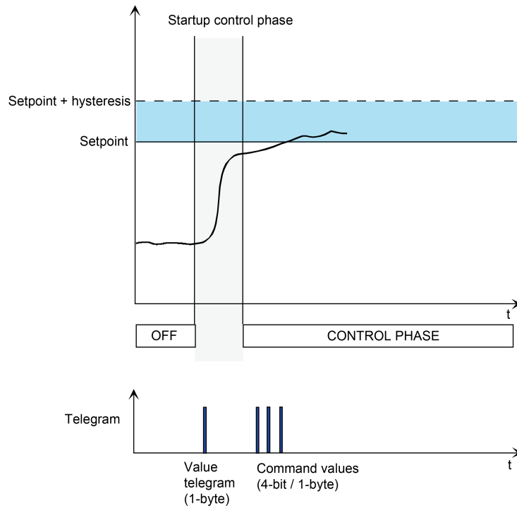
Figure 51: Startup control behaviour with absolute value telegrams (1-byte)
