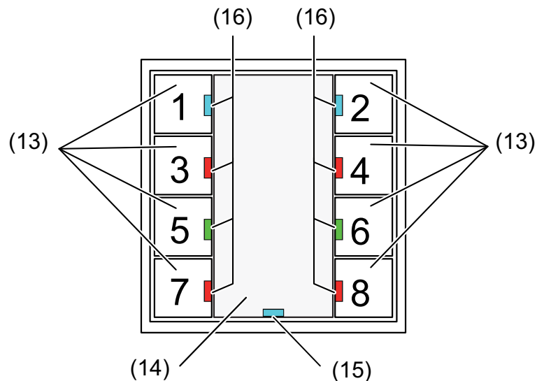
Figure 4: Front view, universal pushbutton sensor module, 4-gang
