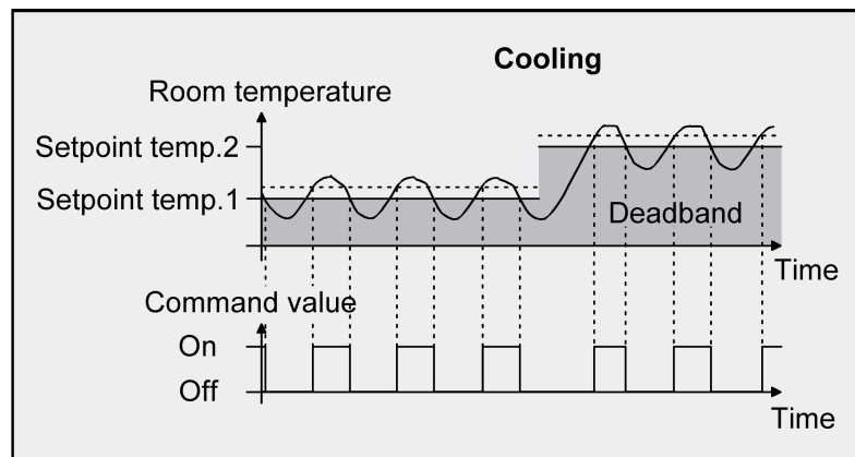
Figure 49: 2-point feedback control for mixed "Heating and cooling" mode with active cooling operation.
