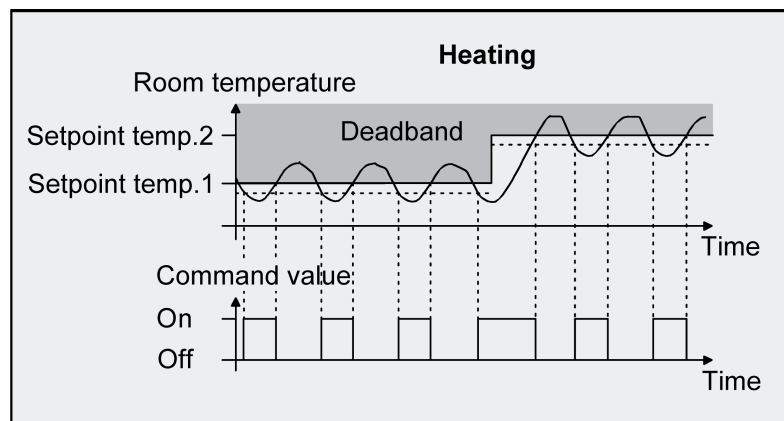
Figure 48: 2-point feedback control for mixed "Heating and cooling" mode with active heating mode.
