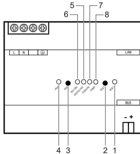
Fig. 4: Operation
