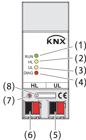
Figure 1: Device components
