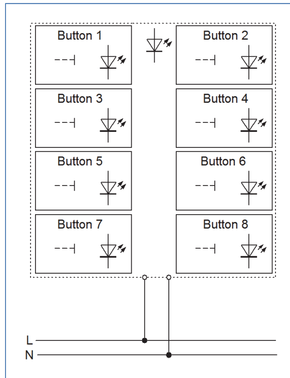
Figure 1: Exemplary circuit diagram RF-TA55P8.01
