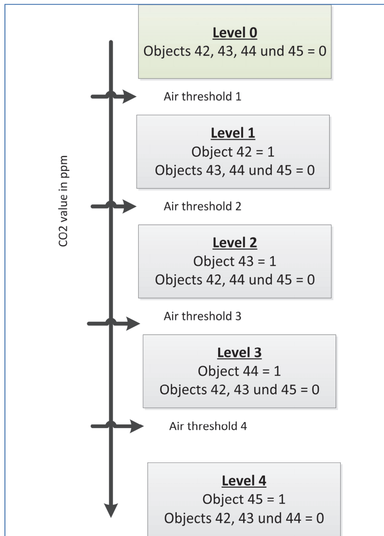
Figure 33: Level controller
