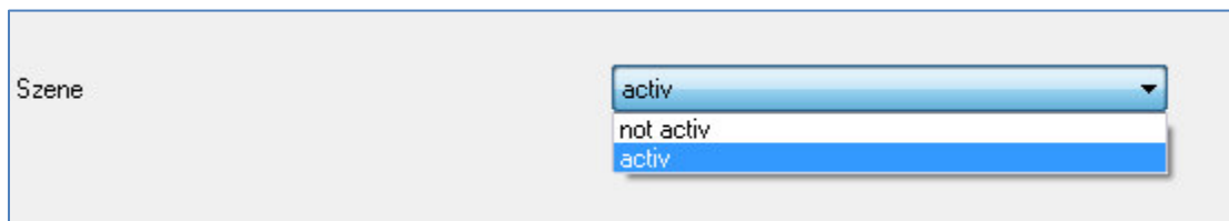
Figure 13: Scene function
