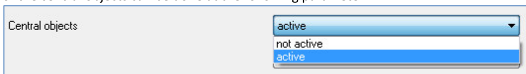
Figure 12: Central objects
