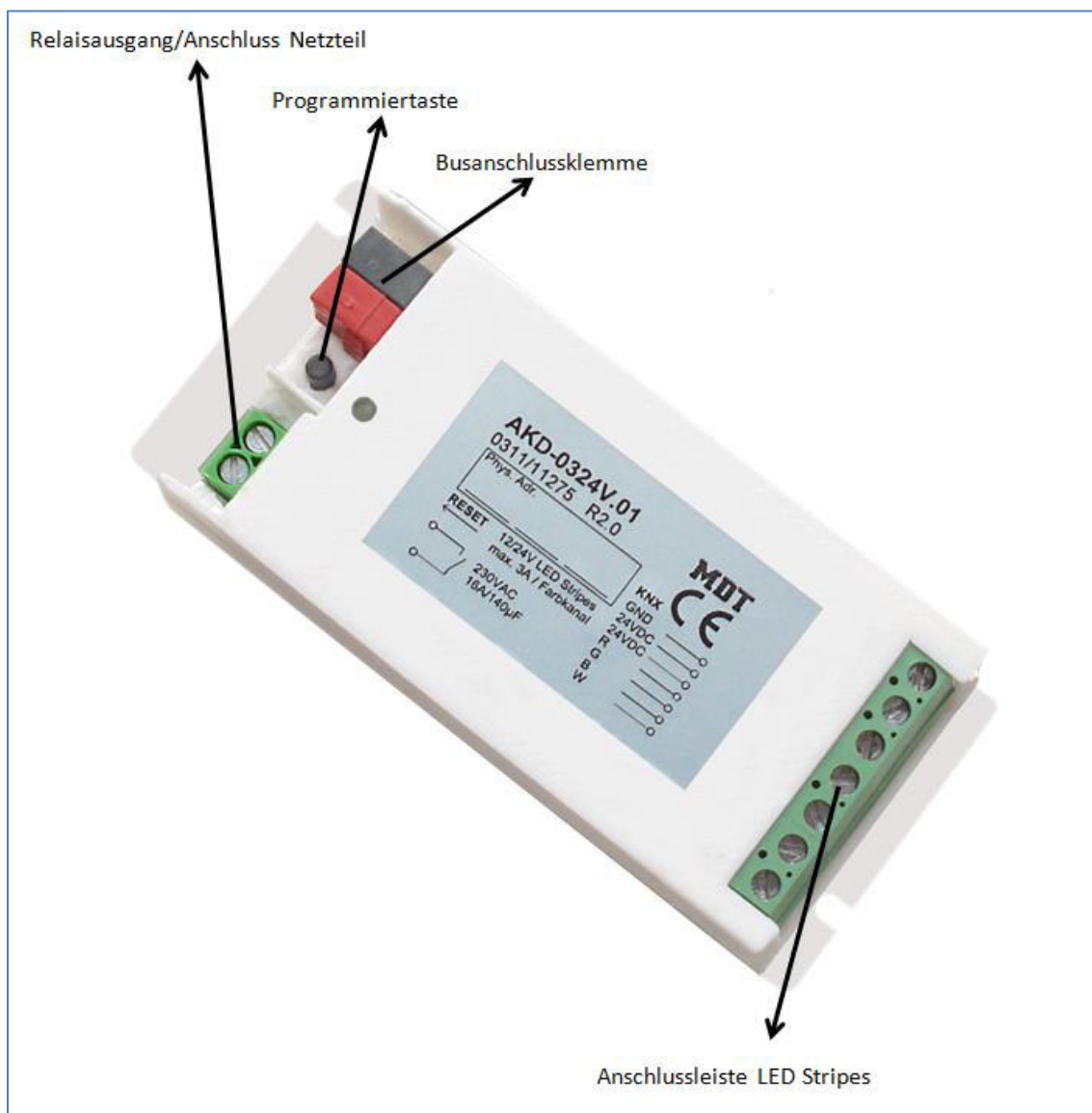
Figure 1: Structure Hardware
