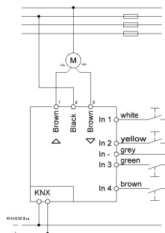
Exemplary circuit diagram AKU-B2UP.03
