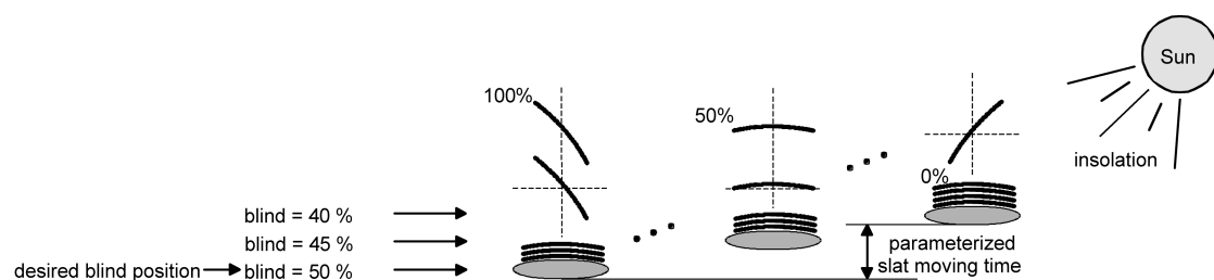
Figure 18: Example of slat positioning affecting the position of the Venetian blind (typical of slat type 1; analogous reaction for type 2)
