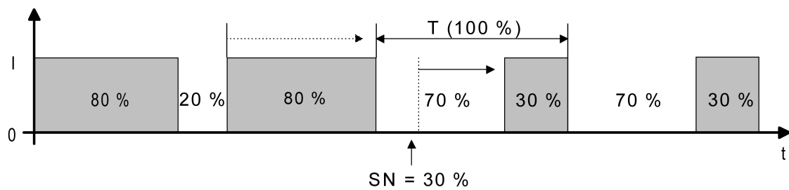
Figure 44: Command value change, e.g. from 80 % to 30 % during the closing phase of the valve
