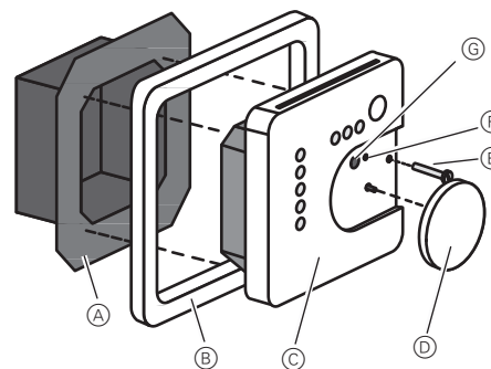
Figure 2: Installing and connecting the device
