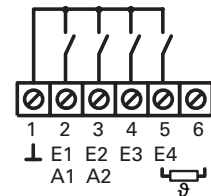
Figure 4: Connect the binary inputs.
