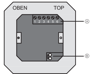
Figure 3: Connect the KNX.
