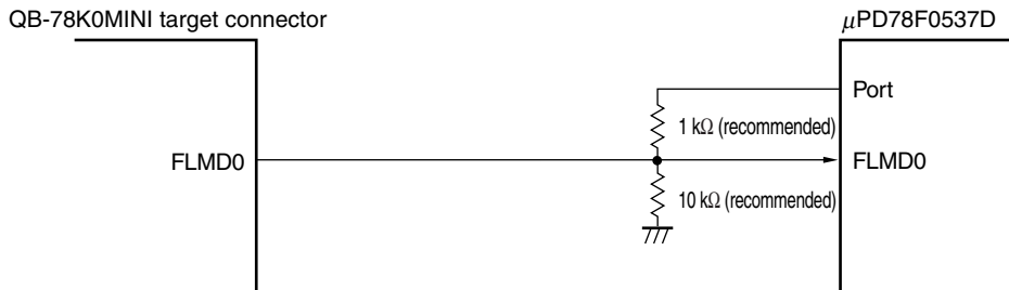
<R> Figure 27-3. Connection of FLMD0 Pin for Self Programming by Means of On-Chip Debugging
