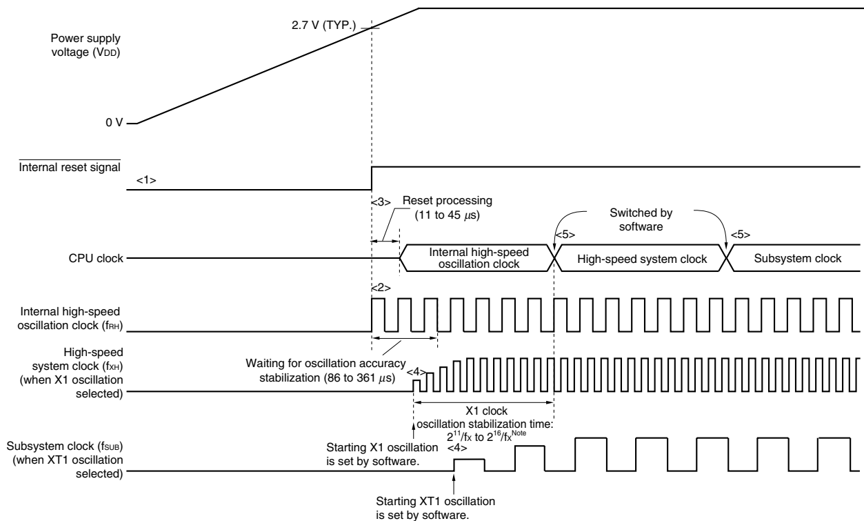
<R> Figure 6-13. Clock Generator Operation When Power Supply Voltage Is Turned On (When 2.7 V/1.59 V POC Mode Is Set (Option Byte: POCMODE = 1))
