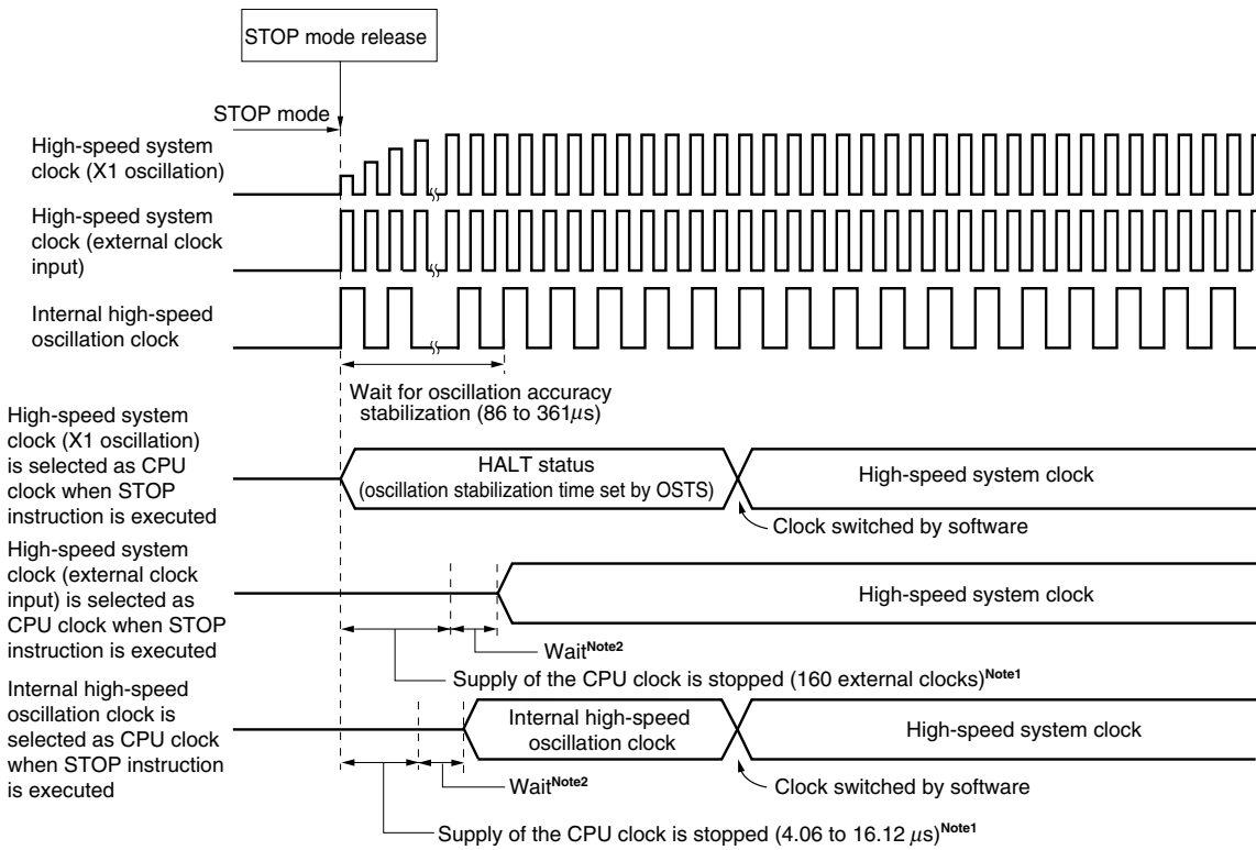
<R> Figure 21-5. Operation Timing When STOP Mode Is Released (When Unmasked Interrupt Request Is Generated)
