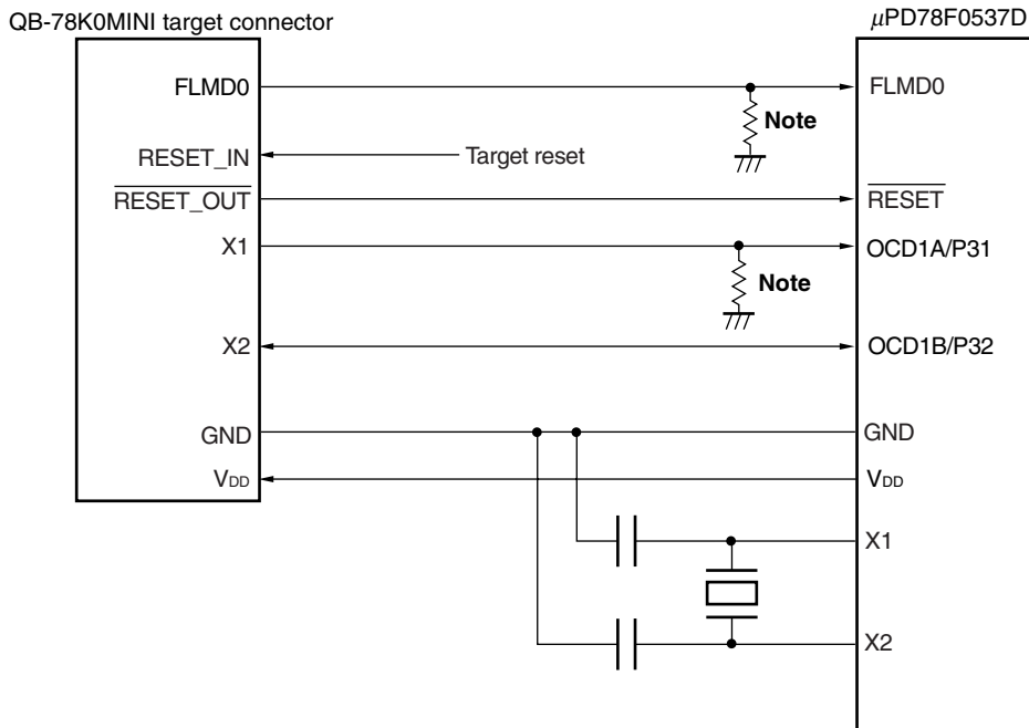
Figure 27-2. Connection Example of QB-78K0MINI and \mu PD78F0537D (When OCD1A/P31 and OCD1B/P32 Are Used)
