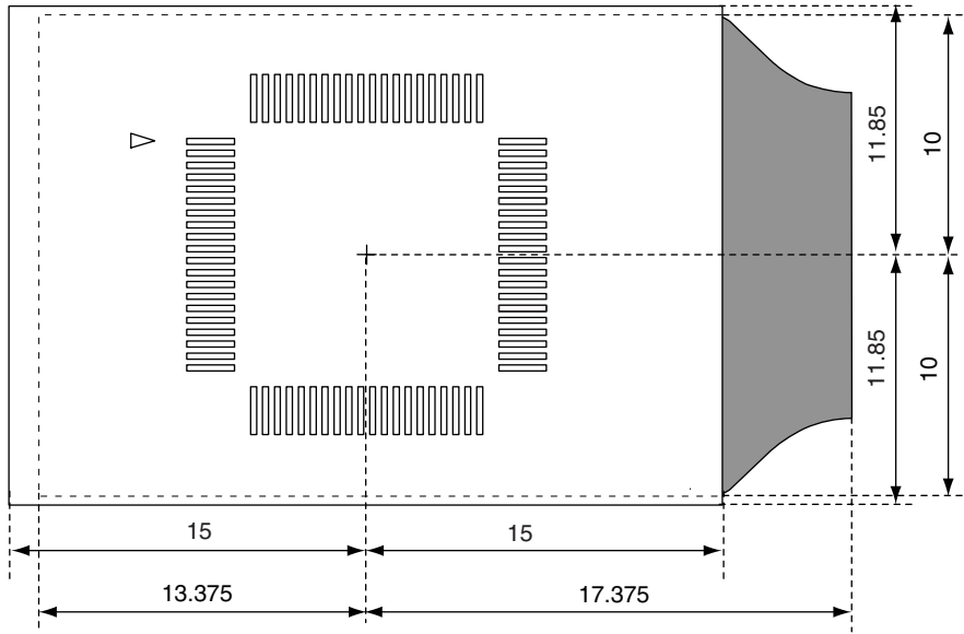
Figure B-4. For 64-Pin GC Package
