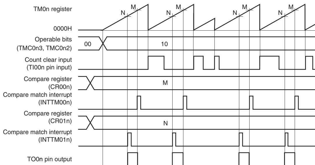
(b) TOC0n = 13H, PRM0n = 10H, CRC0n, = 00H, TMC0n = 0AH
