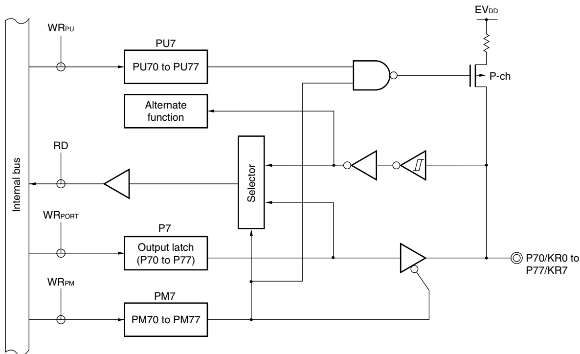
Figure 5-21. Block Diagram of P70 to P77
