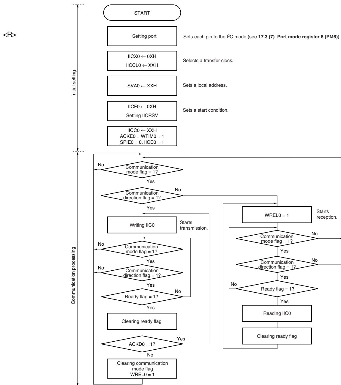
Figure 17-25. Slave Operation Flowchart (1)
