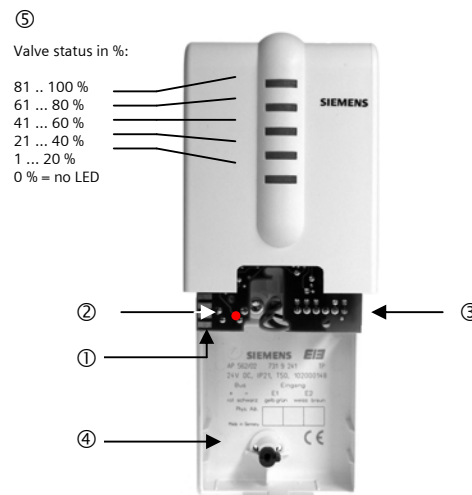
figure 1: Location of the Display and Operating Elements
