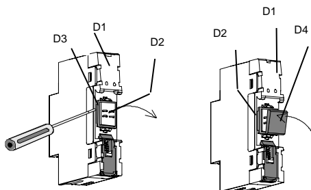
Figure 2: Covering the contact system
