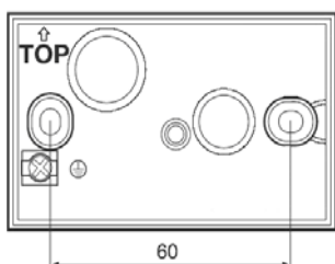
Figure 6: Correct position of the connection box
