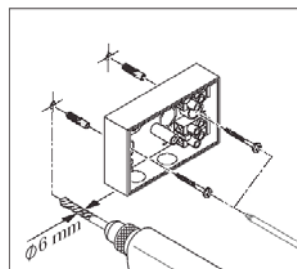
Figure 7: Mounting the connection box
