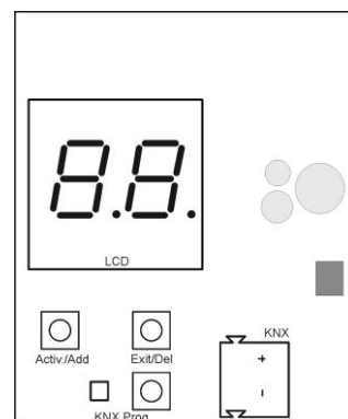
Fig. 3: Device with top open
