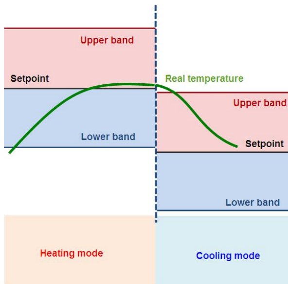
Figure 27. Automatic mode switching due to setpoint change
