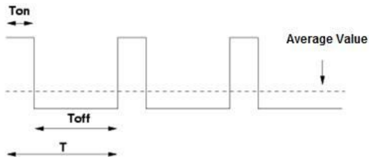
Figure 4. Value of variable PI equal to 25%.
