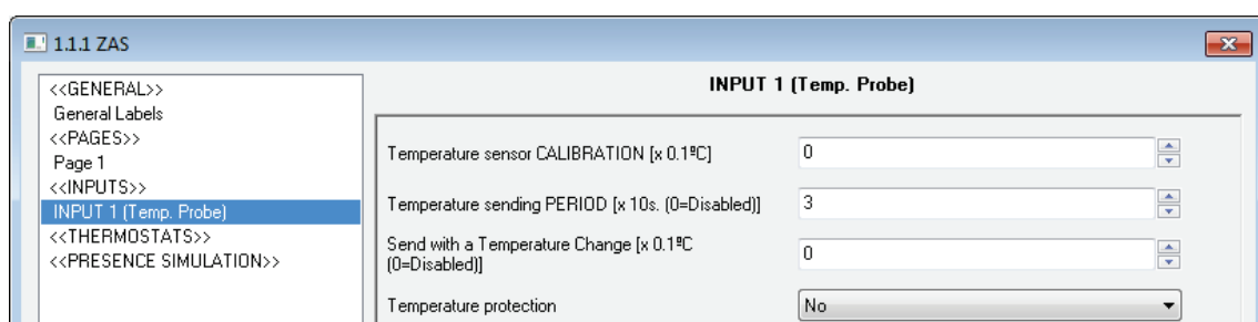
Figure 22. Input: temperature probe
