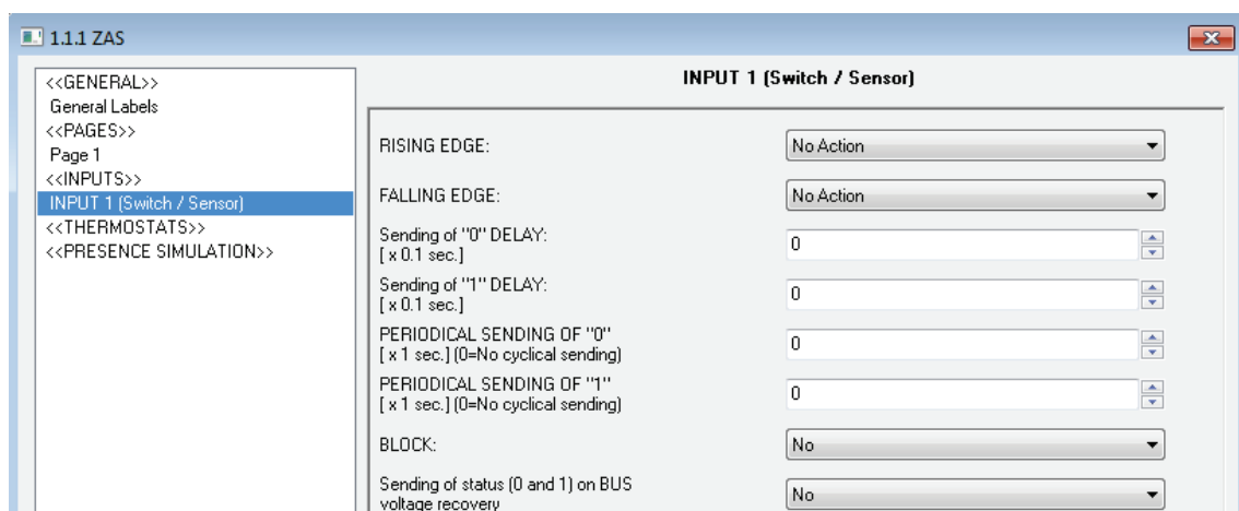
Figure 21. Input: switch/sensor
