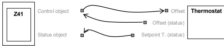
Figure 52 Relative (float) setpoint control. Object linking.
