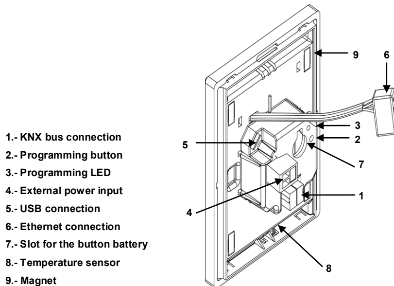
Figure 1 Element diagram
