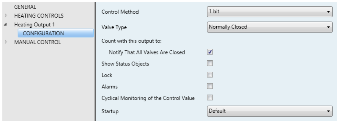
Figure 7. Heating Control – Configuration.
