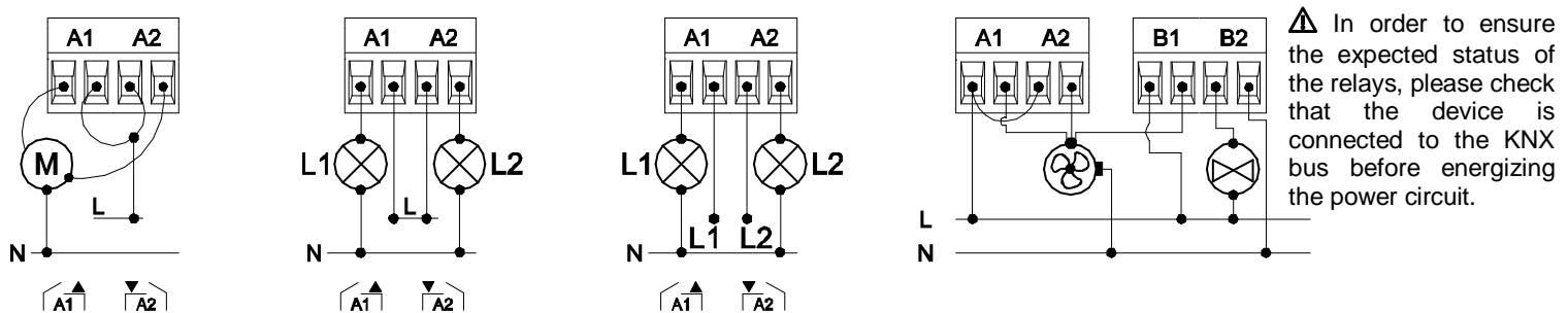
Figure 2. Wiring examples (from left to right): channel A as shutter channel, individual outputs in channel A with the same and different phases and channel A and B as fan coil controller (2 pipe and three-speed fan).
