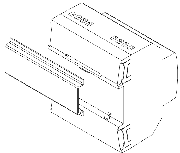
Figure 3. Installation of MAXinBOX 8 Plus on DIN rail
