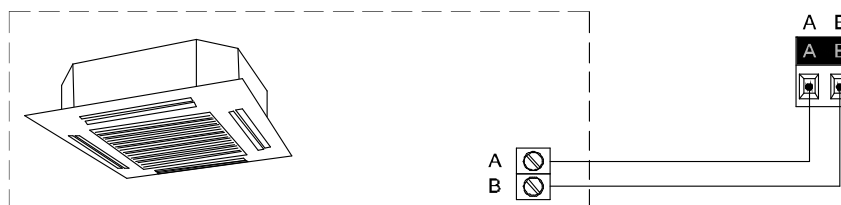
Figure 2. Wiring KLIC-TS to the Air Conditioning Equipment
